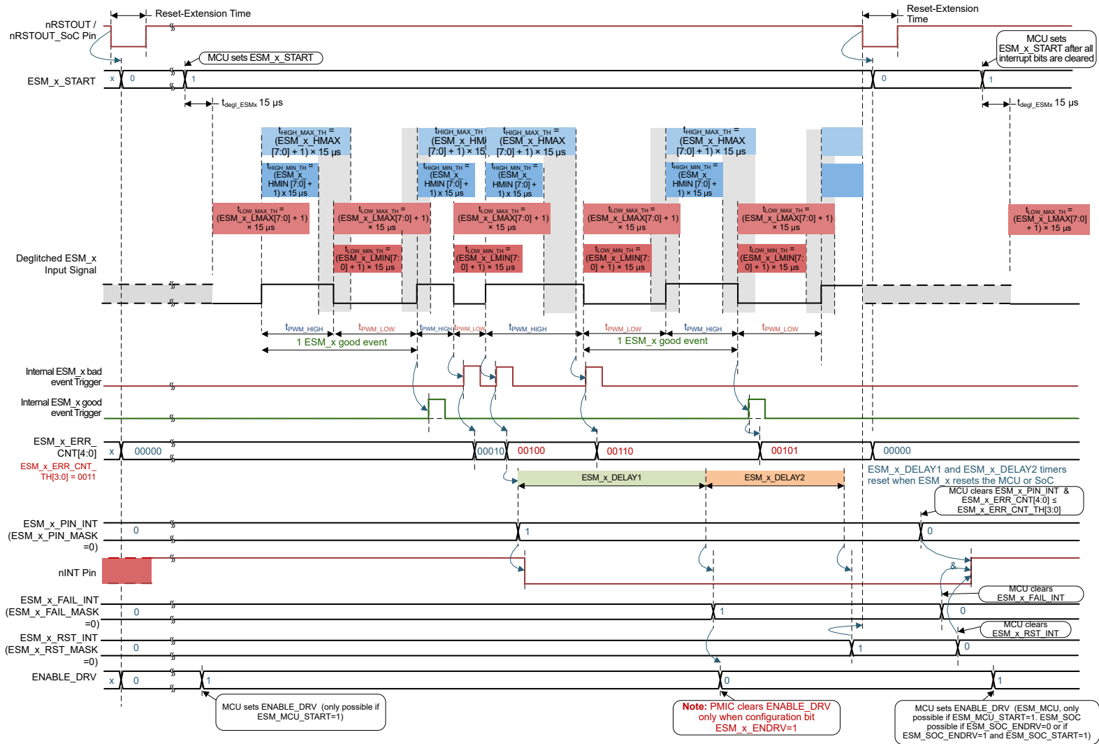
Case Number 4: _DELAY2 > 0 PWM signal has an error after start-up, and the ESM_x_ERR_CNT[4:0] > ESM_x_ERR_CNT_TH[3:0] during the elapse of ESM_x_DELAY1 and ESM_x_DELAY2 . Hence the PMIC pulls the nRSTOUT / nRSTOUT_SoC pin low, and releases this pin after the reset-extension time. After this, MCU clears all errors and restarts the ESM_x .
