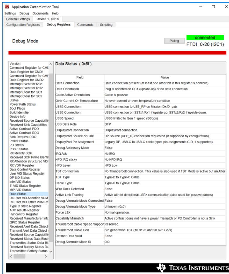
Figure 7. Data Status Register Read from TPS65987D Acting as DFP_D
