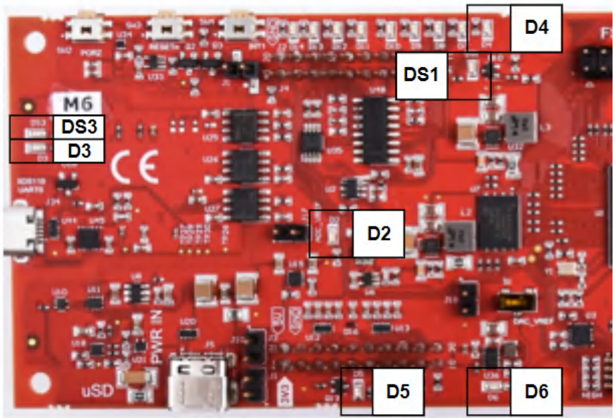
Figure 3-2. Power Status LEDs
