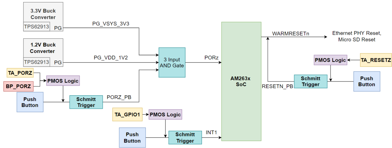
Figure 4-2. Reset Architecture
