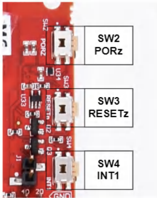
Figure 3-4. Push Buttons
