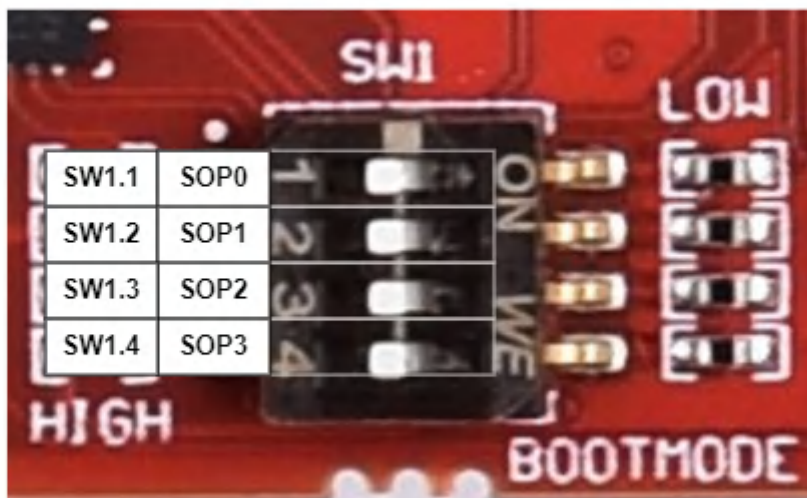
Figure 3-5. Bootmode DIP Switch Positions
