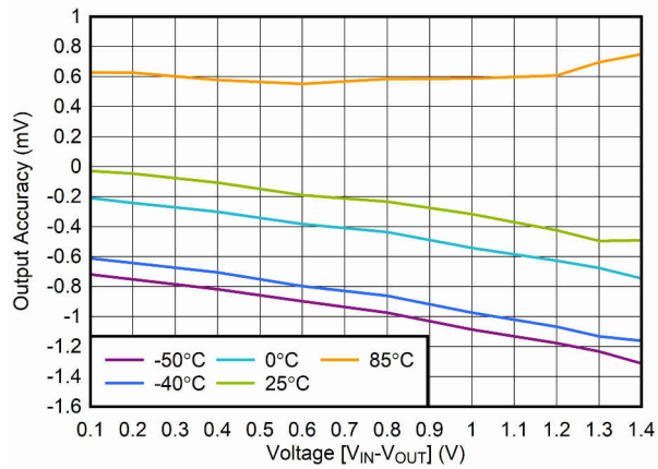
Figure 6-1. Output Voltage Accuracy vs V_{\text{IN}}
