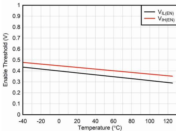
Figure 6-11. Enable Threshold vs Temperature
