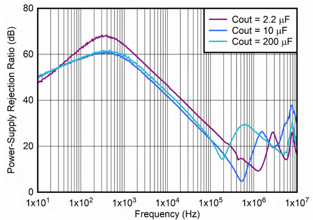
Figure 6-24. PSRR vs Frequency and C_{OUT}
