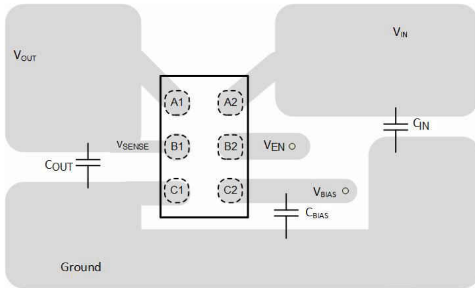
Figure 10-1. Recommended Layout
