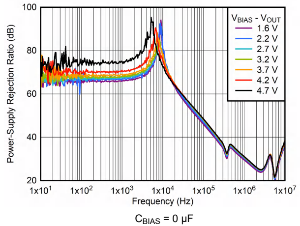
Figure 6-26. PSRR vs Frequency and V_{BIAS} - V_{OUT}
