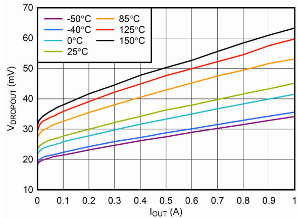
Figure 6-4. V_{\text{IN}} Dropout Voltage vs I_{\text{OUT}}
