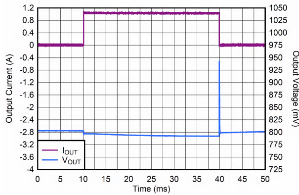
Figure 6-21. Load Transient From 100 \mu\text{A} to 1 A
