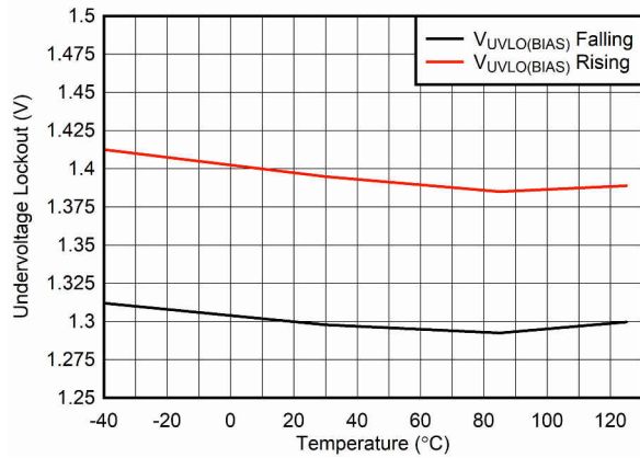
Figure 6-13. V_{BIAS} UVLO vs Temperature
