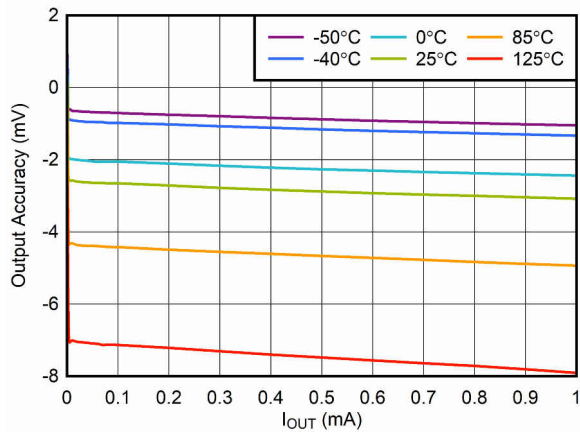
Figure 6-3. Output Voltage Accuracy vs I_{\text{OUT}}
