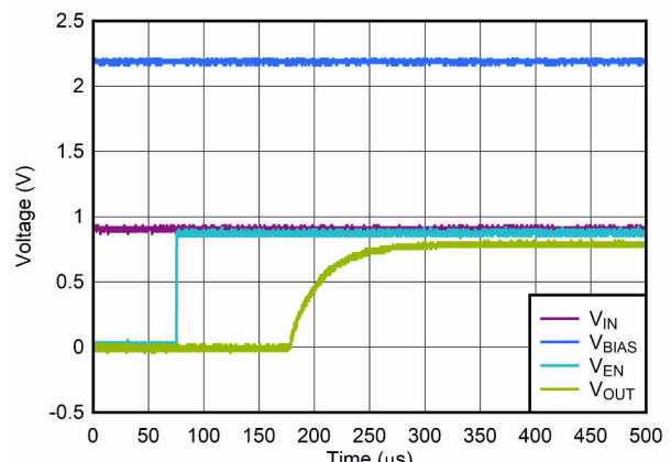
Figure 6-14. Start-Up With V_{BIAS} Before V_{IN}
