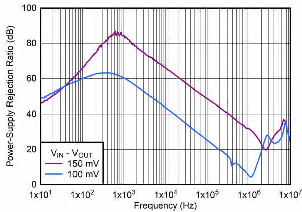
Figure 6-23. PSRR vs Frequency and V_{IN} - V_{OUT}
