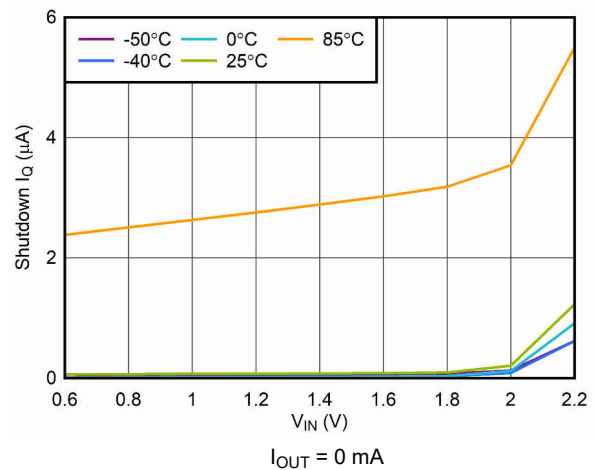
Figure 6-8. V_{\text{IN}} Shutdown I_Q vs V_{\text{IN}}
