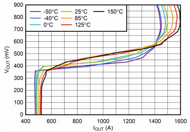
Figure 6-10. V_{\text{OUT}} Foldback Current Limit vs Output Current
