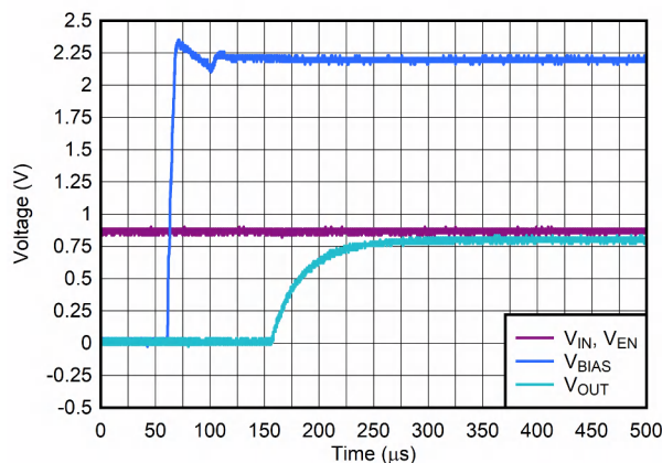
Figure 6-17. Start-Up With V_{IN} and V_{EN} Before V_{BIAS}
