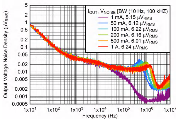
Figure 6-27. Output Noise vs Frequency and I_{OUT}
