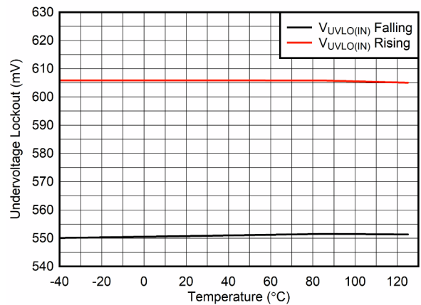
Figure 6-12. V_{\text{IN}} UVLO vs Temperature
