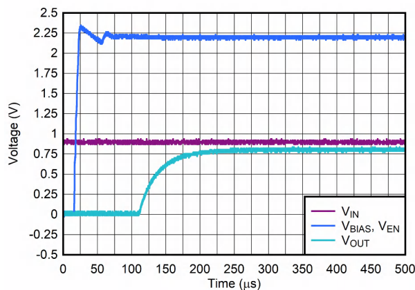
Figure 6-15. Start-Up With V_{IN} Before V_{BIAS} and V_{EN}
