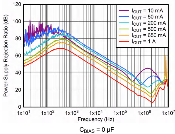
Figure 6-25. PSRR vs Frequency and I_{OUT}
