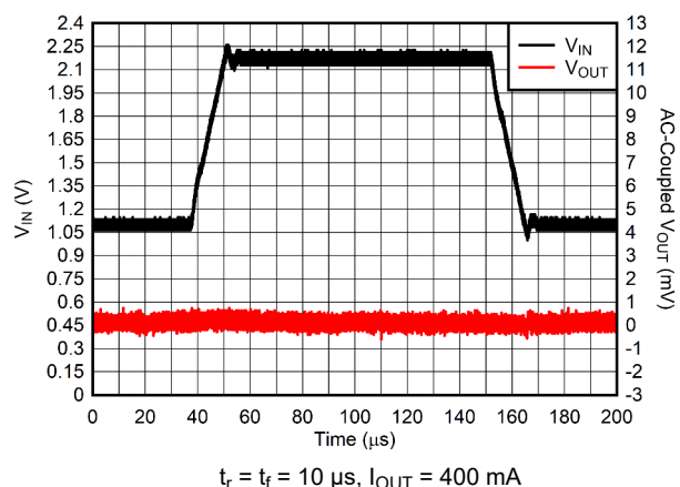
Figure 6-18. Line Transient From 1 V to 2.2 V
