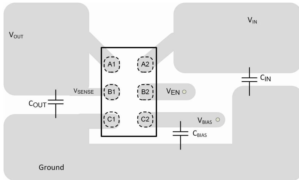
Figure 8-6. Recommended Layout
