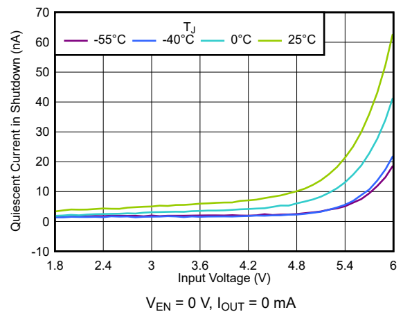
Figure 6-12. Shutdown Current vs V_{IN}
