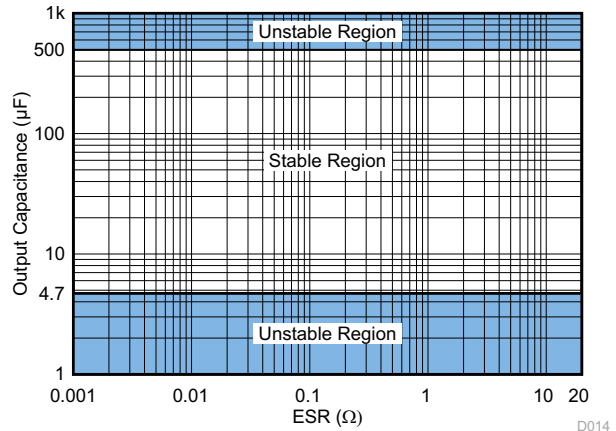
Figure 6-14. ESR Stability vs Output Capacitance
