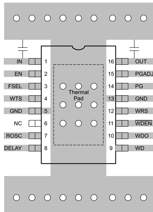
Figure 10-1. Layout Recommendation
