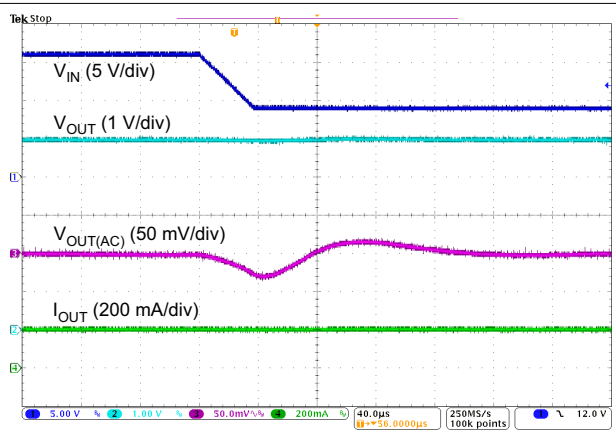
Figure 6-16. Line Transient
