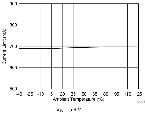
Figure 6-9. Output Current Limit ( I_{LIM} ) vs Ambient Temperature
