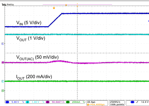
Figure 6-15. Line Transient
