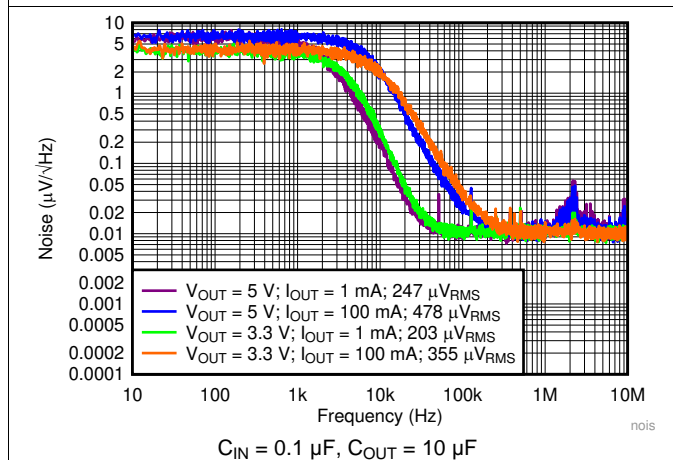
Figure 23. Noise vs Frequency
