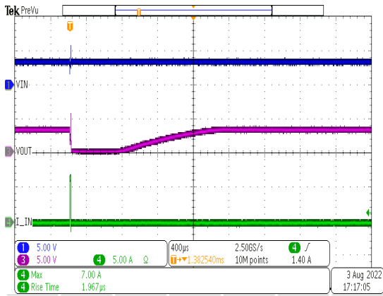
Figure 6-27. Hot Short Event when ON and Recovery
