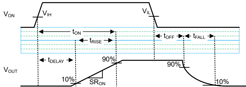
Figure 7-2. Timing Waveforms
