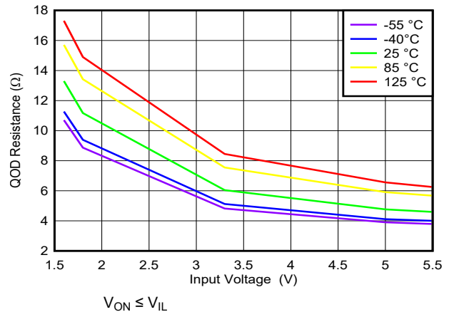
Figure 6-6. QOD Resistance vs Input Voltage
