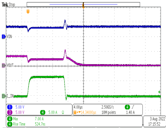
Figure 6-26. Hot Short Event when ON
