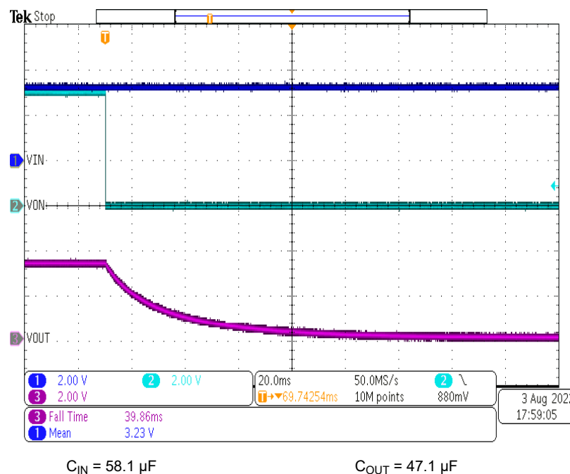
Figure 9-2. Fall Time ( R_{ODD} = 1\text{ k}\Omega )
