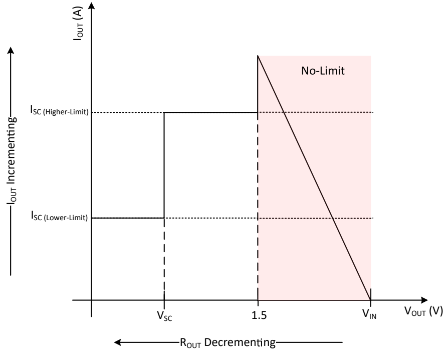
Figure 8-1. Output Short Circuit Current Limit
