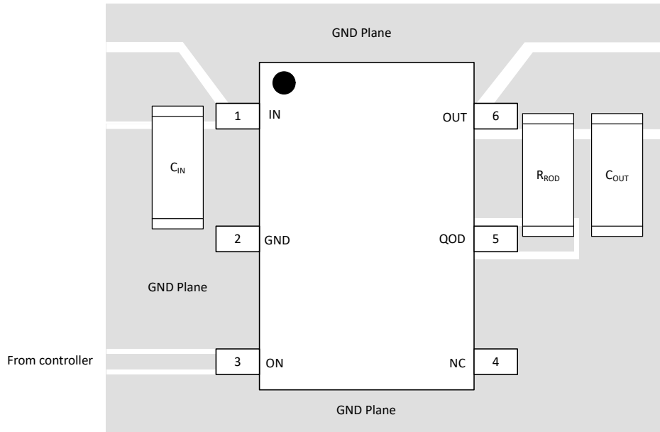
Figure 11-1. Recommended Board Layout
