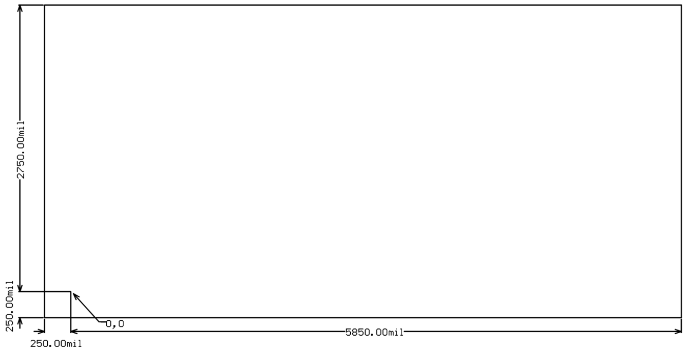
Figure 7-14. PCB Dimensions
