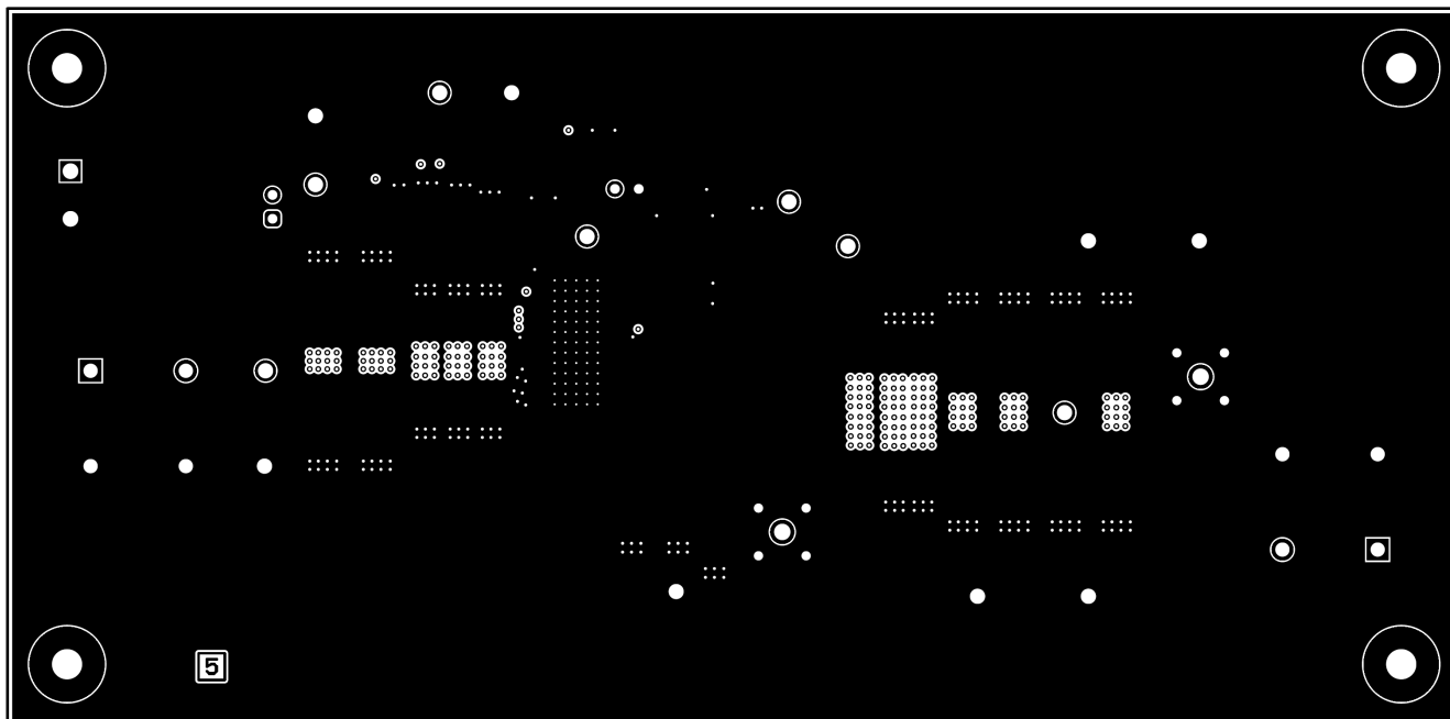
Figure 7-7. Signal Layer Four
