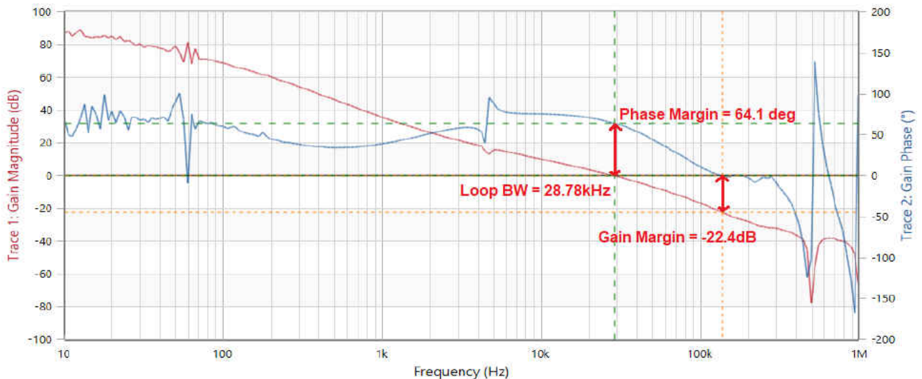
Figure 4-8. Frequency Response
