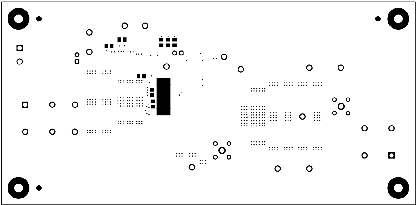
Figure 7-11. Bottom Solder
