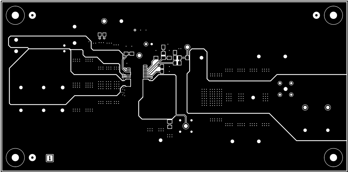
Figure 7-3. Top Layer
