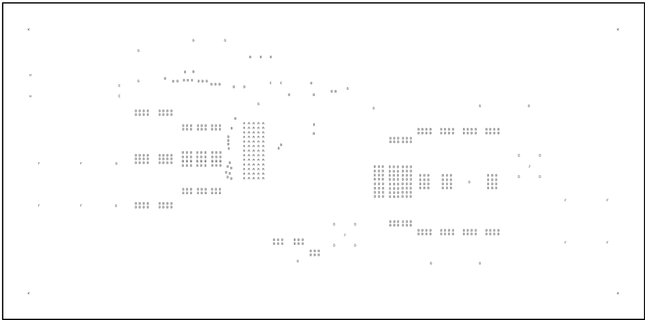
Figure 7-13. Drill Drawing
