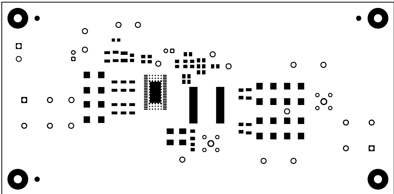
Figure 7-2. Top Solder
