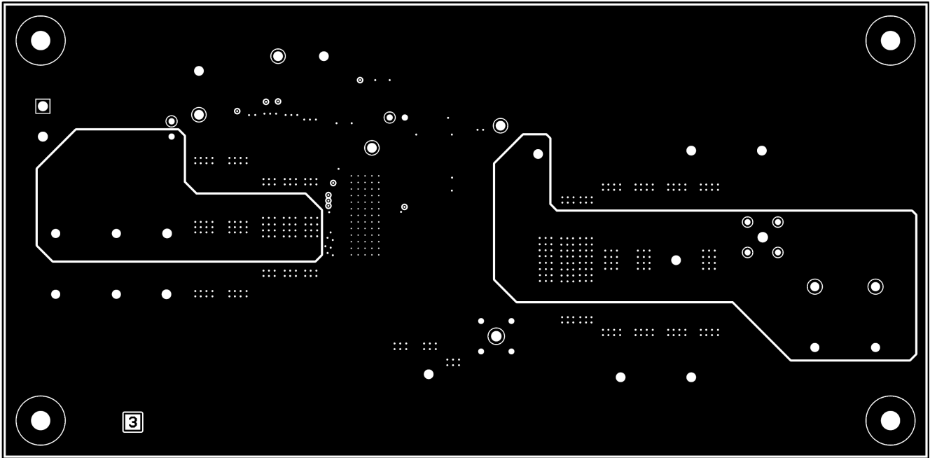
Figure 7-5. Signal Layer Two
