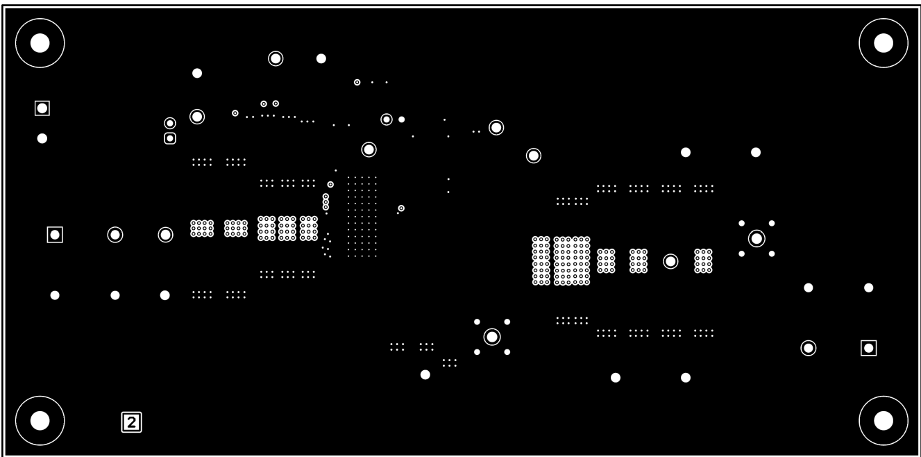
Figure 7-4. Signal Layer One
