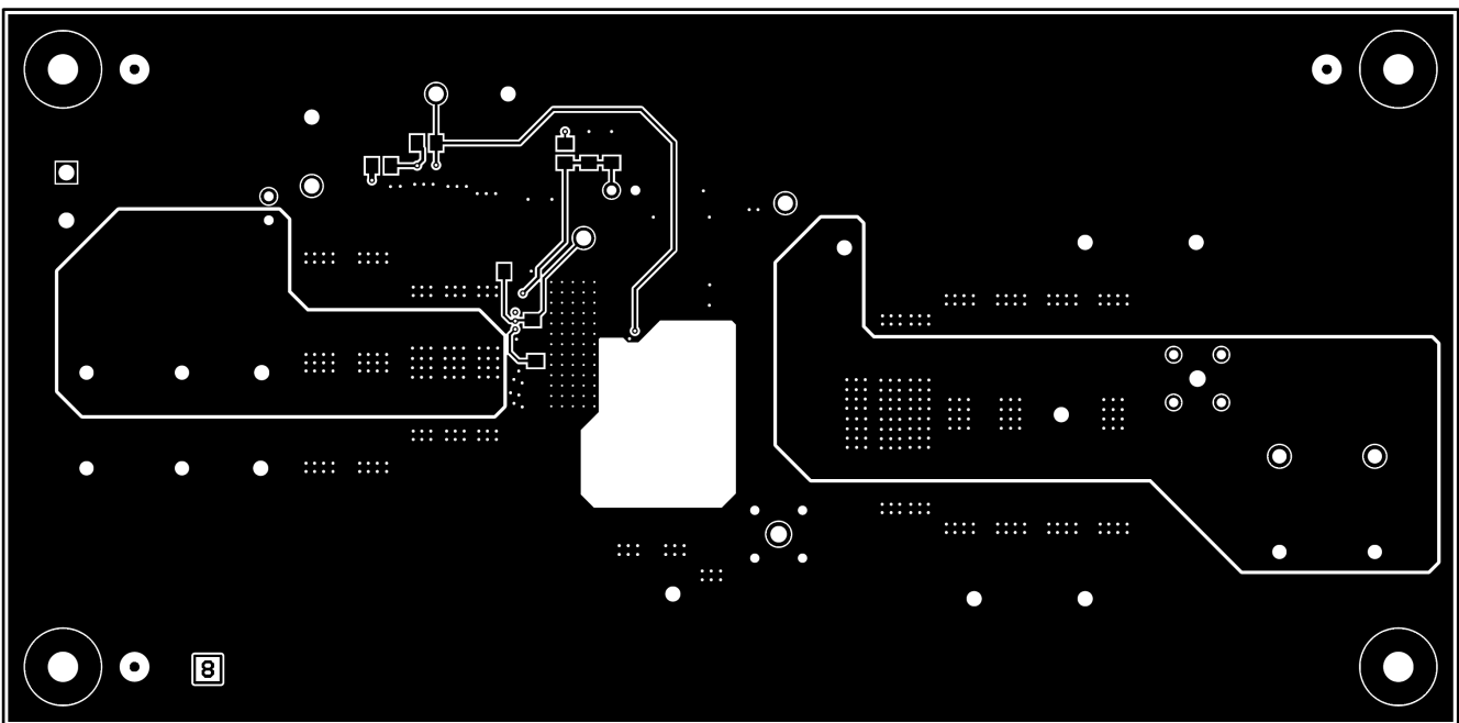
Figure 7-10. Bottom Layer
