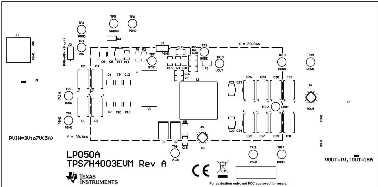
Figure 7-1. Top Overlay
