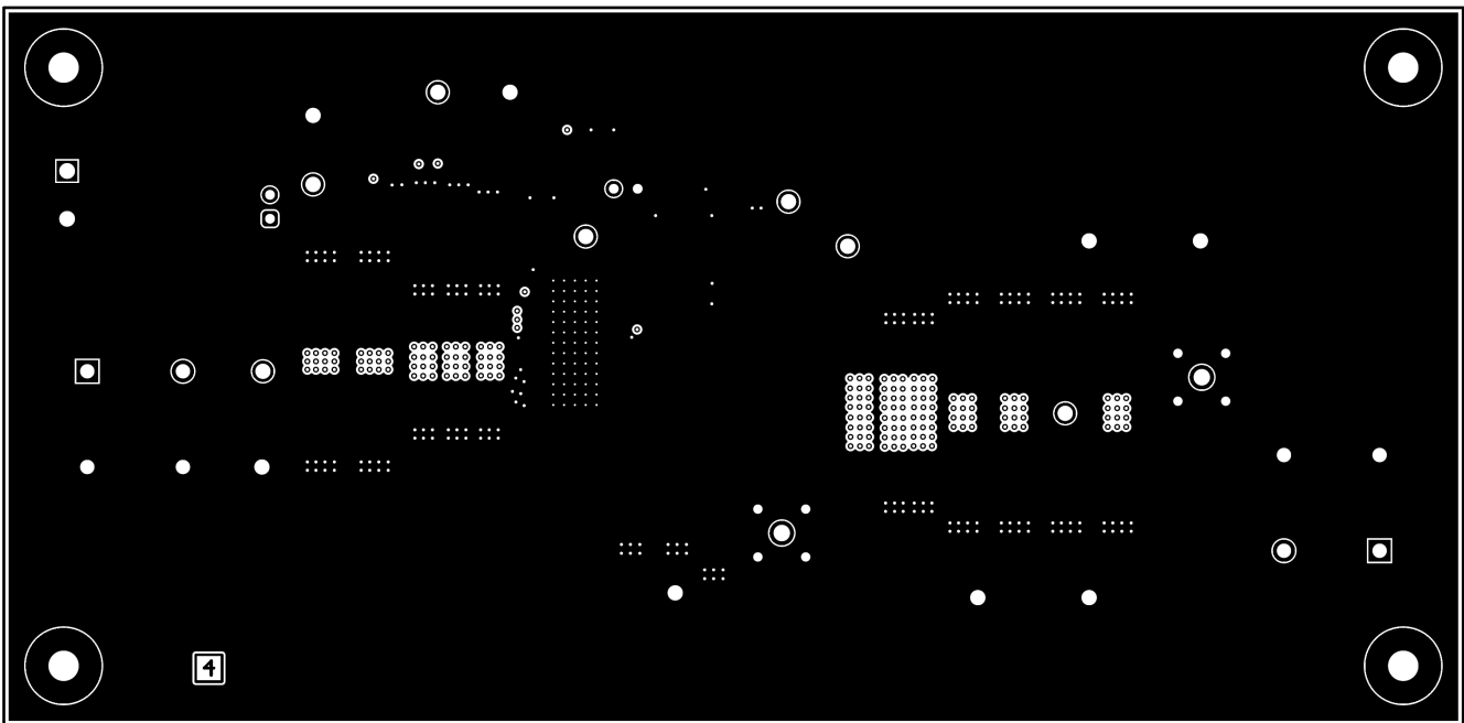
Figure 7-6. Signal Layer Three
