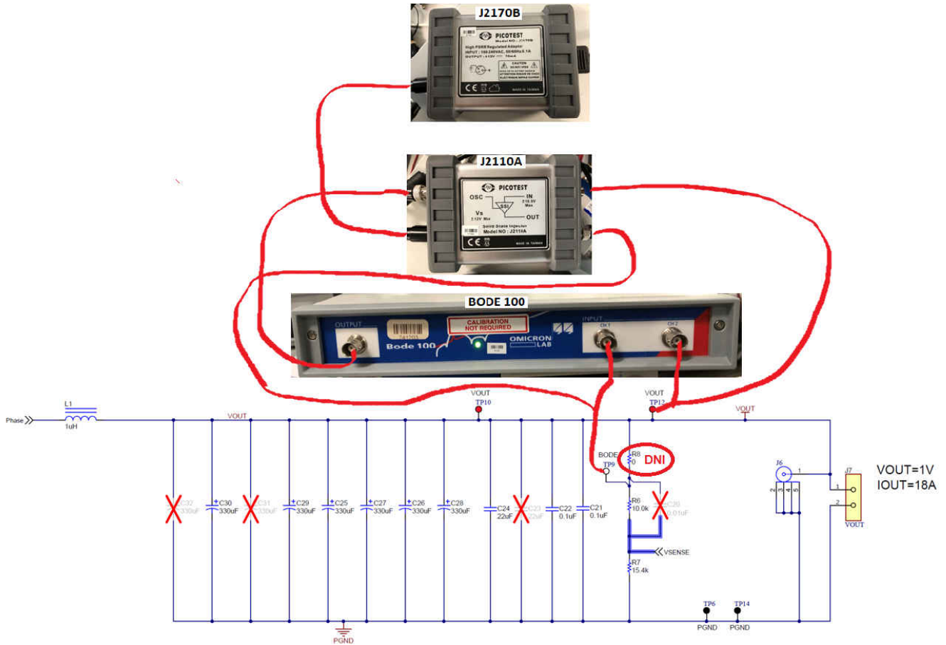
Figure 4-7. Frequency Response Test Setup
