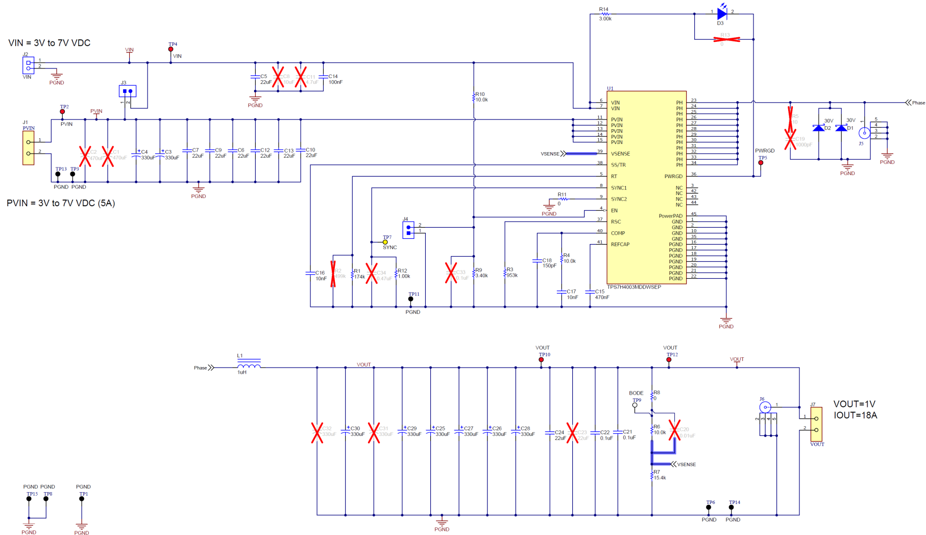
Figure 5-1. TPS7H4003EVM Schematic
