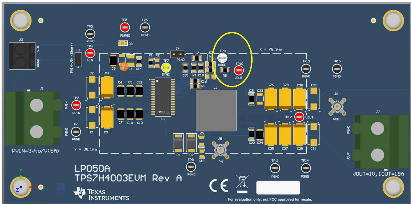
Figure 4-6. EVM Modification to Measure Frequency Response
