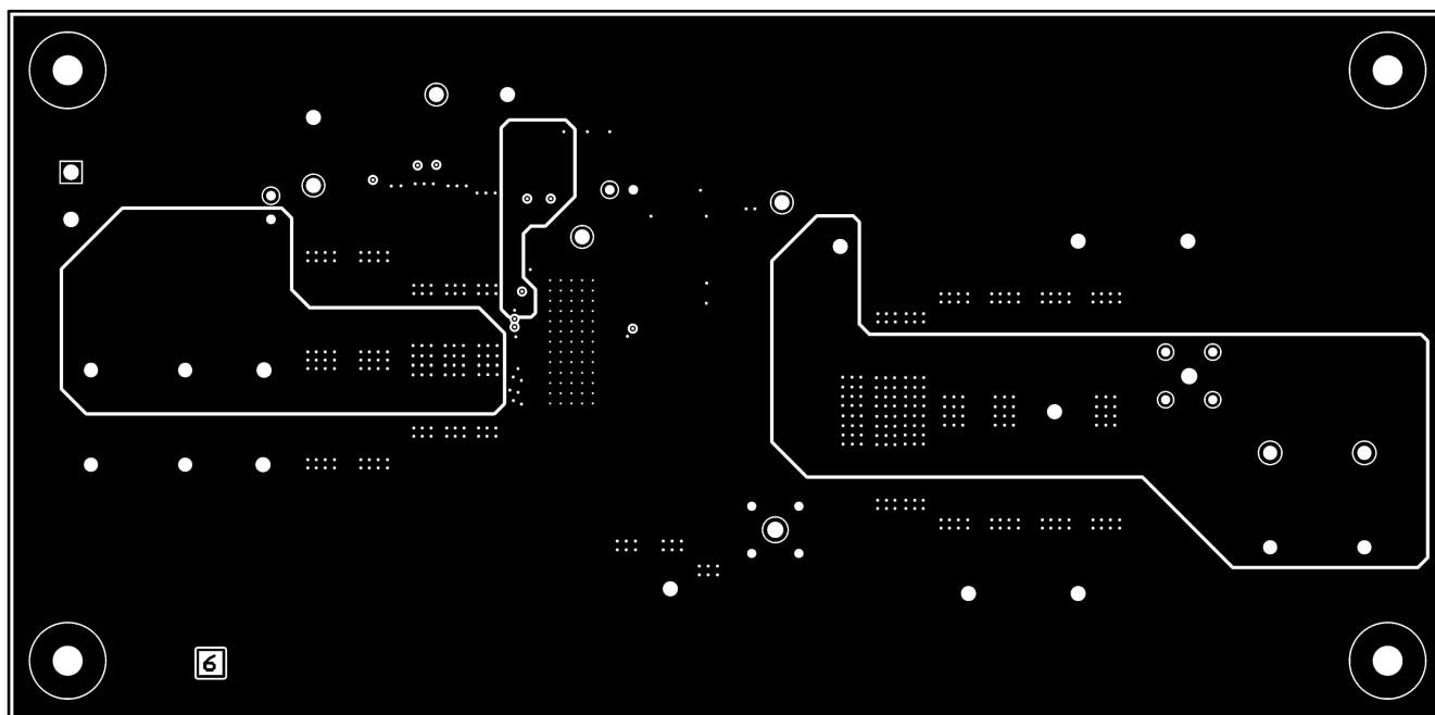
Figure 7-8. Signal Layer Five
