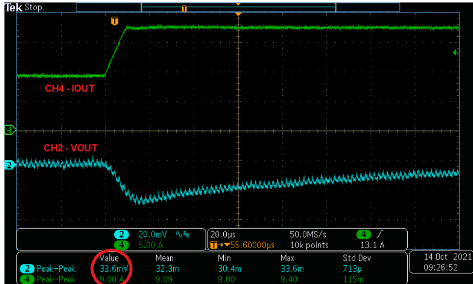
Figure 4-4. Transient Response to Load Step 9 A to 18 A at 1 A/μs
