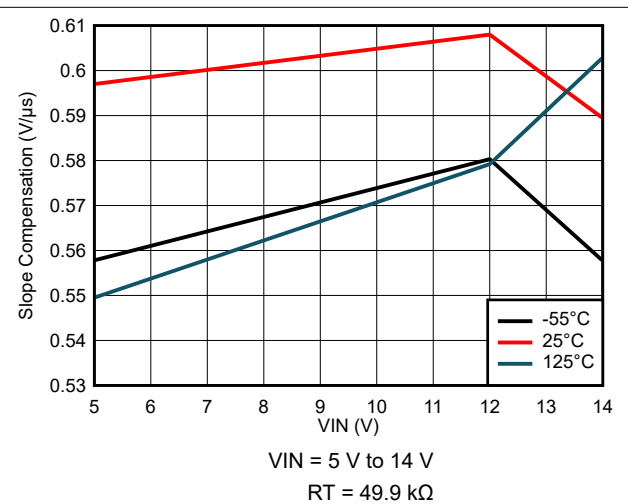
Figure 7-72. Slope Compensation Variation
