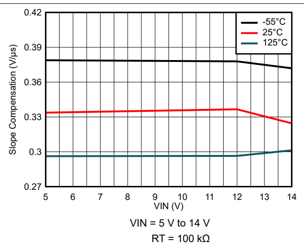
Figure 7-70. Slope Compensation Variation
