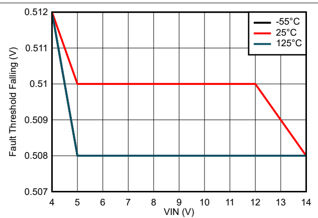
Figure 7-32. FAULT Threshold Falling Variation
