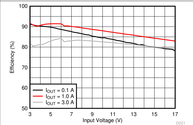
Figure 8-7. Efficiency, V_{OUT} = 2.5\text{ V}
