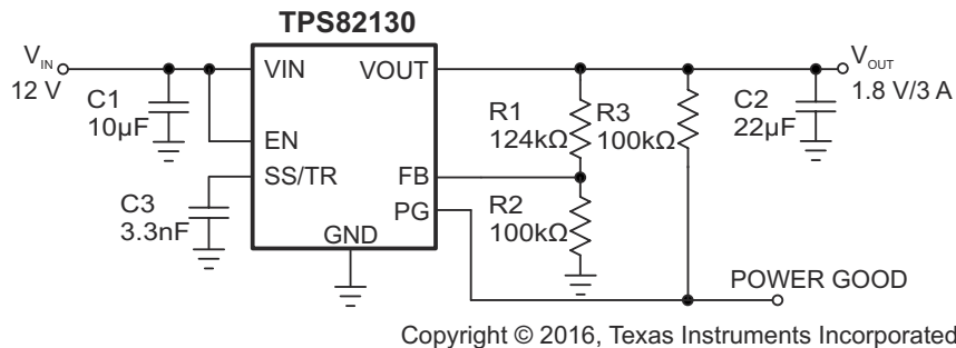
Figure 8-1. 1.8-V Output Application
