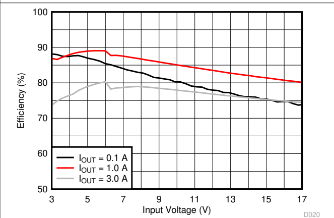
Figure 8-5. Efficiency, V_{OUT} = 1.8\text{ V}
