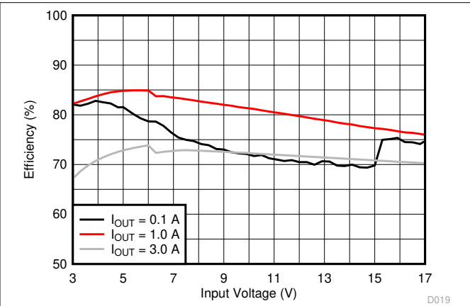
Figure 8-3. Efficiency, V_{OUT} = 1.0\text{ V}
