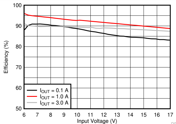
Figure 8-11. Efficiency, V_{OUT} = 5.0\text{ V}
