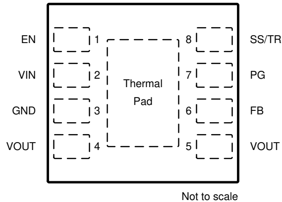
Figure 5-1. 8-Pin µSiL Package (SIL0008C Top View)
