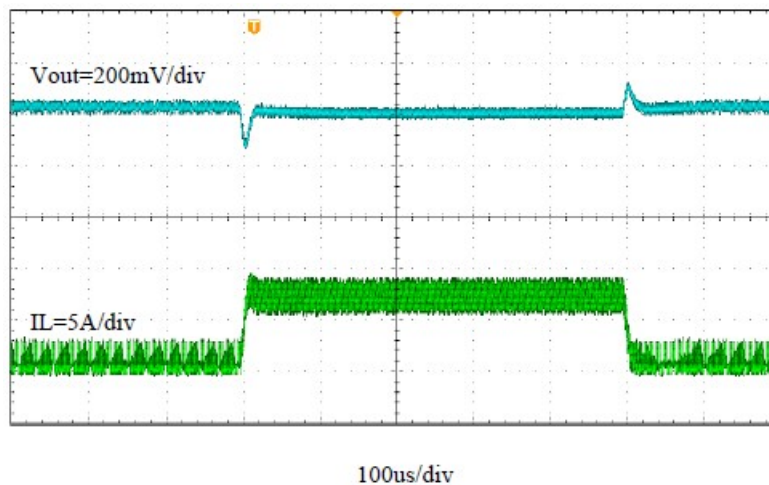
Figure 4-1. TPS51395 Transient Waveform
