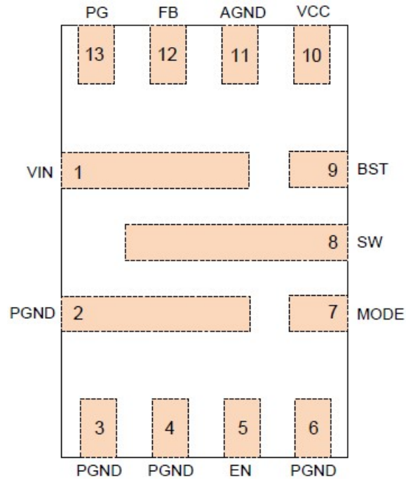
Figure 5-1. TPS566335 in 2x3mm QFN Package
