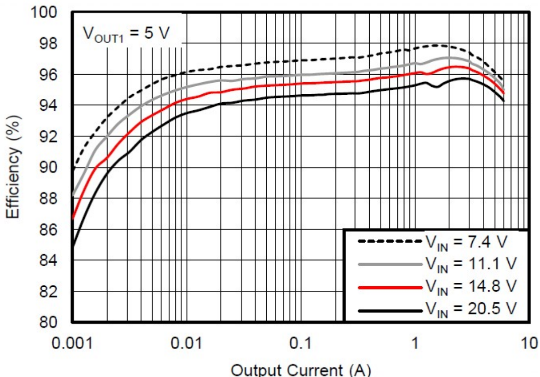
Figure 2-1. TPS51285A Efficiency Plot
