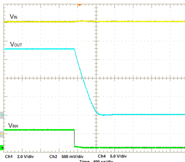
Figure 3. Shut Down Waveform (using INH)
