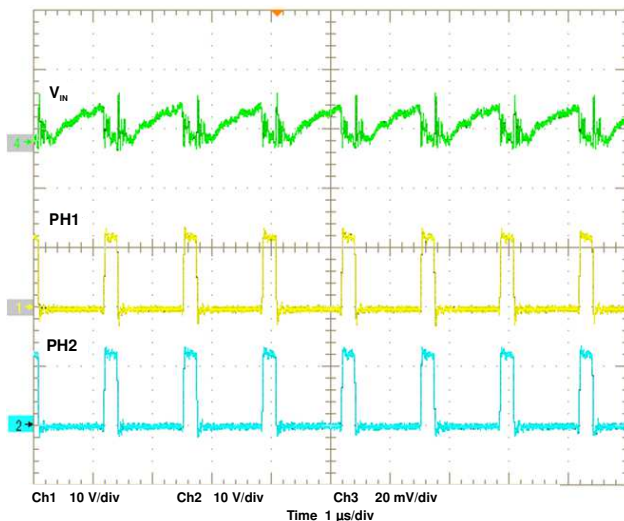
Figure 7. Input Voltage Ripple In-Phase
