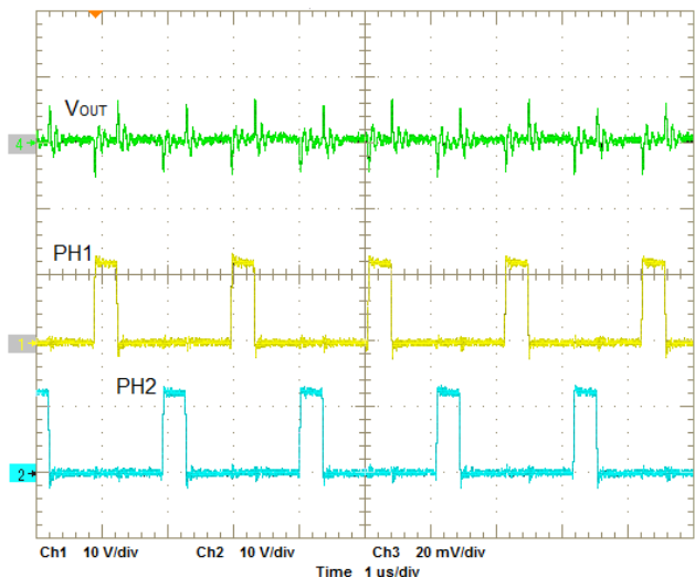
Figure 6. Output Voltage Ripple 180^\circ Out-of-Phase
