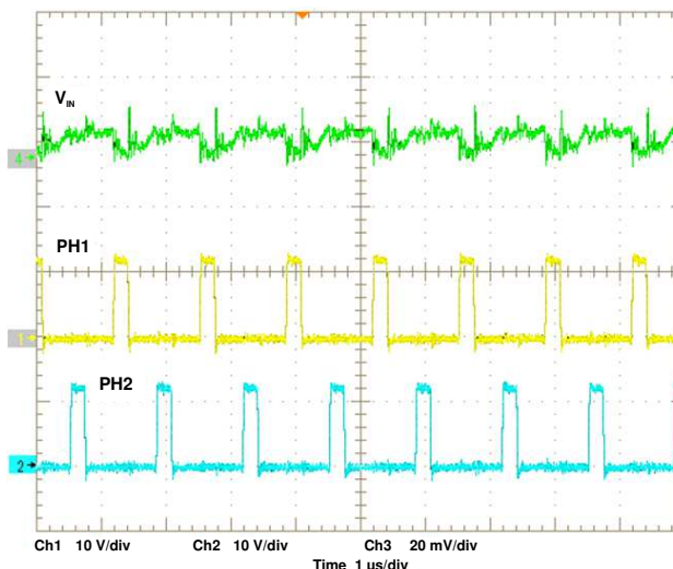
Figure 8. Input Voltage Ripple 180^\circ Out-of-Phase
