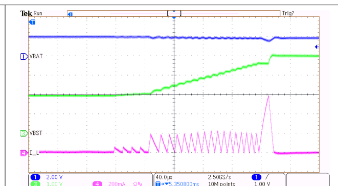
Figure 9-3. Boost Soft-Start
