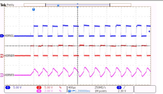
Figure 9-9. 3-Terminal Horn Driver Waveforms
