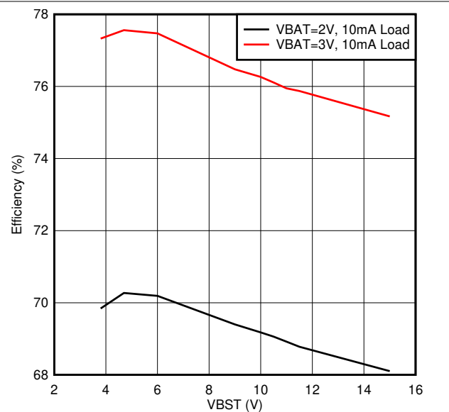
Figure 9-5. Boost Converter Efficiency
