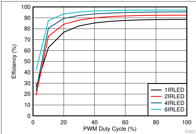
Figure 6-15. Efficiency at 1-A Output Current, 4.7- \mu\text{H} Inductor, 12-V Input Voltage
