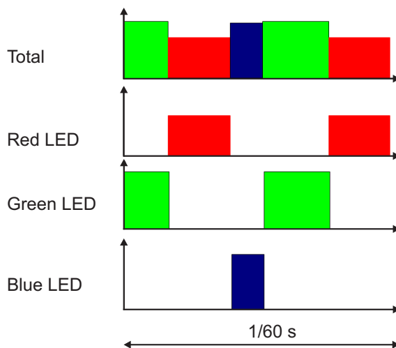
Figure 2. Conventional LED Driving Scheme in 60 Hz Video
