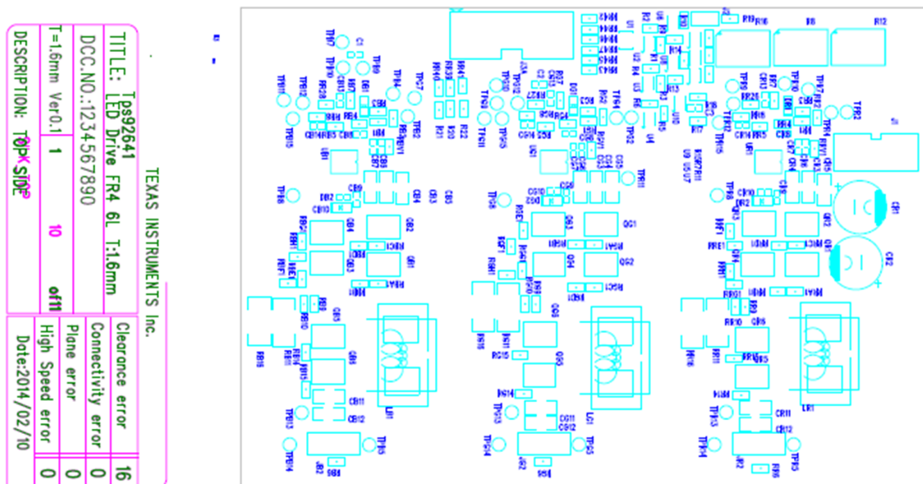
Figure 17. PCB Top View With Component
