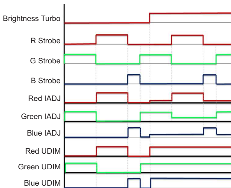
Figure 7. Logic Chart of Brightness Turbo Inputs/Outputs
