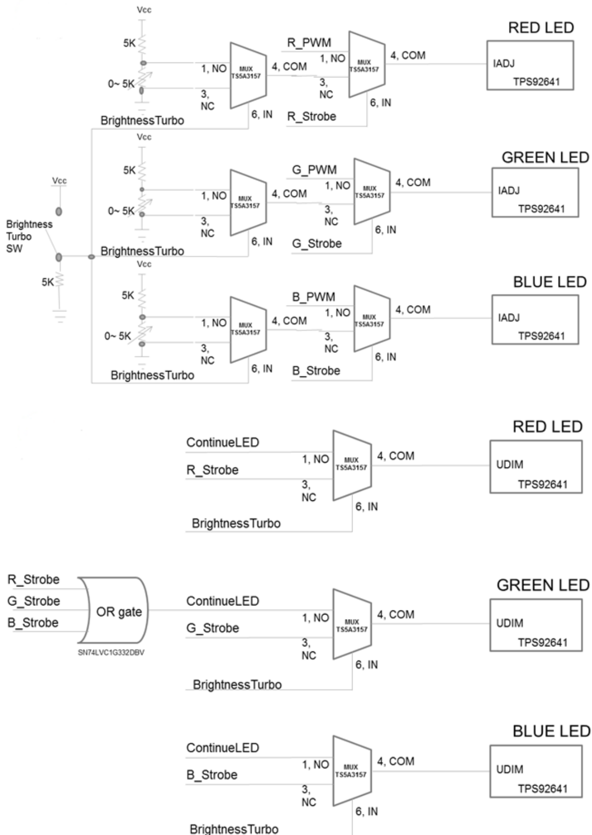
Figure 8. Brightness Turbo Circuit for R, G, B Channels
