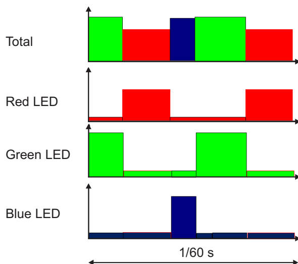
Figure 3. Brightness Turbo Slightly Turned on all LEDs at all Times
