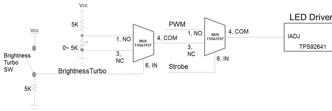
Figure 4. IADJ Control of Brightness Turbo
