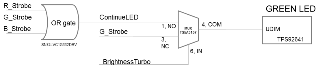
Figure 6. UDIM Control on Green LED
