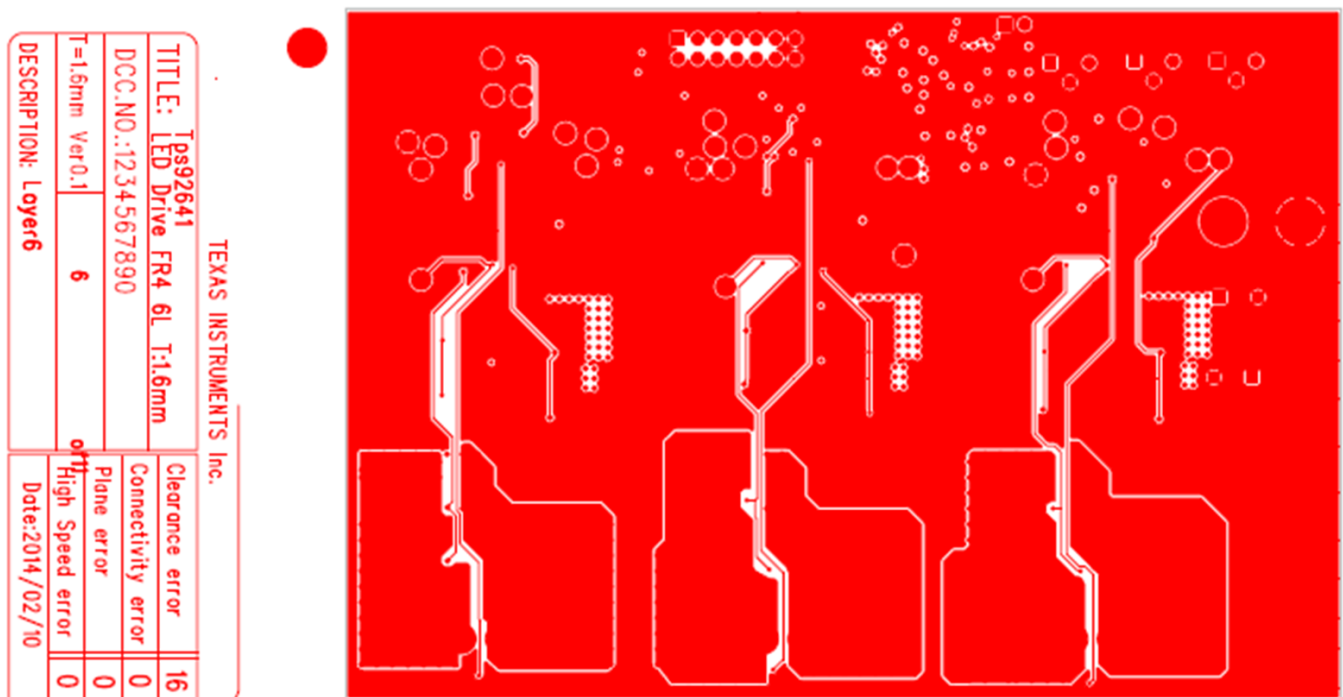
Figure 16. Bottom View
