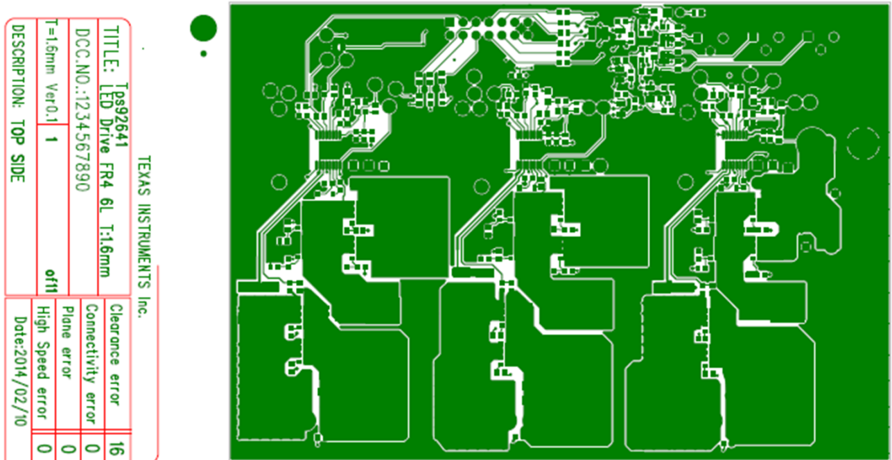
Figure 15. Top View
