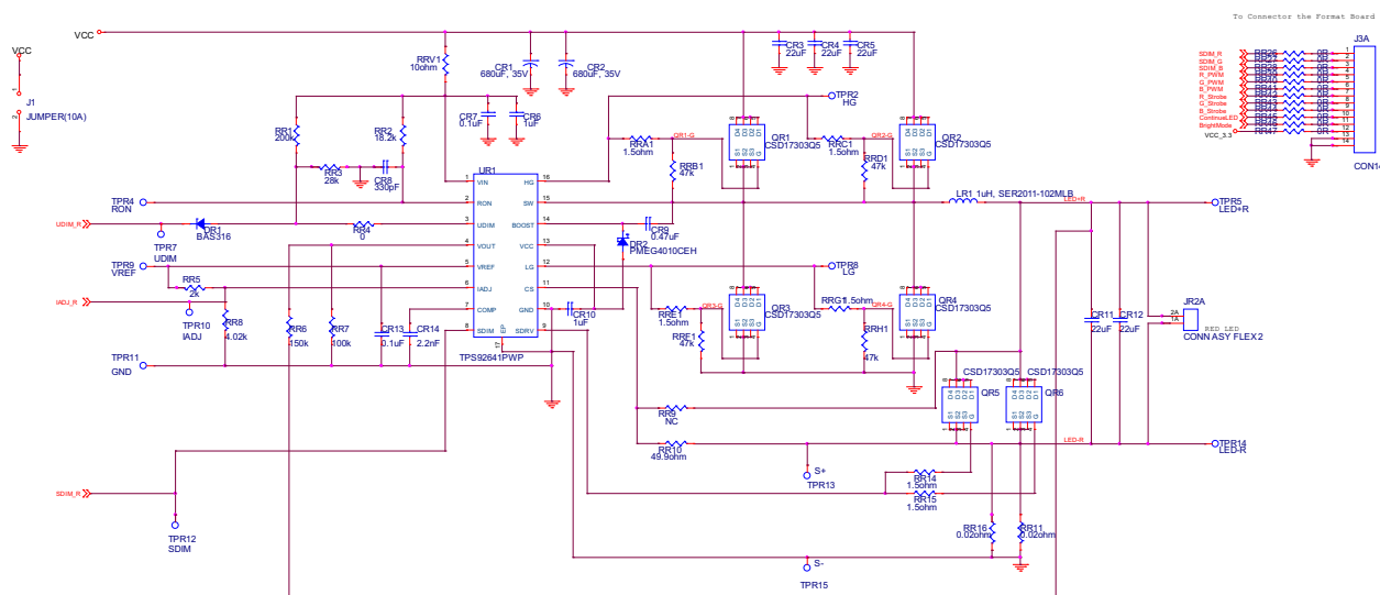
Figure 11. TPS92641 Red LED Driver Schematic
