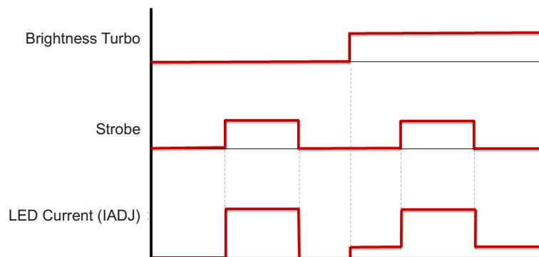
Figure 5. Logic Chart of Control over IADJ
