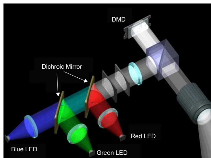
Figure 1. Optical Layout of DLP® LED Projector
