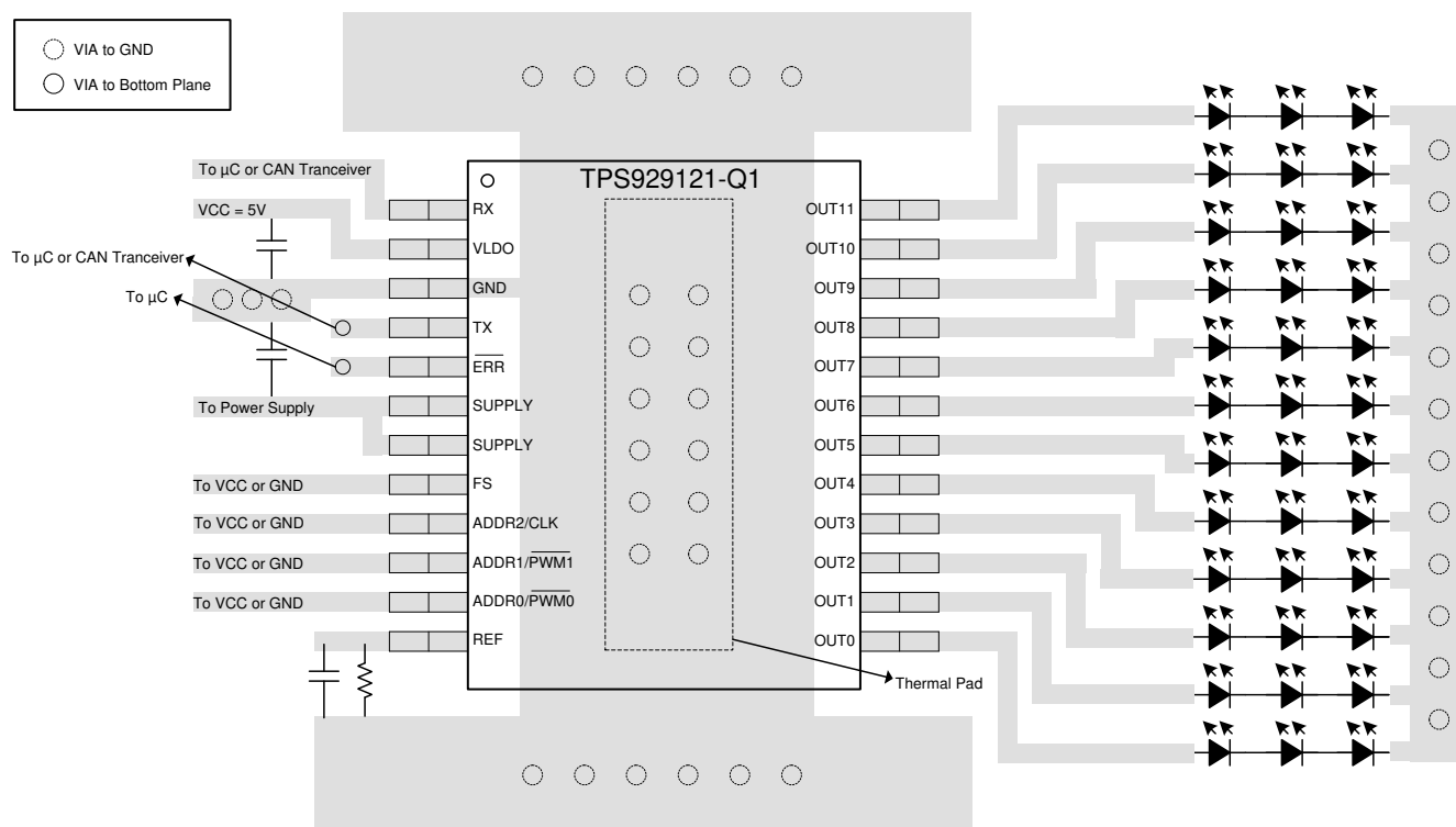
Figure 11-1. TPS929121-Q1 Layout
