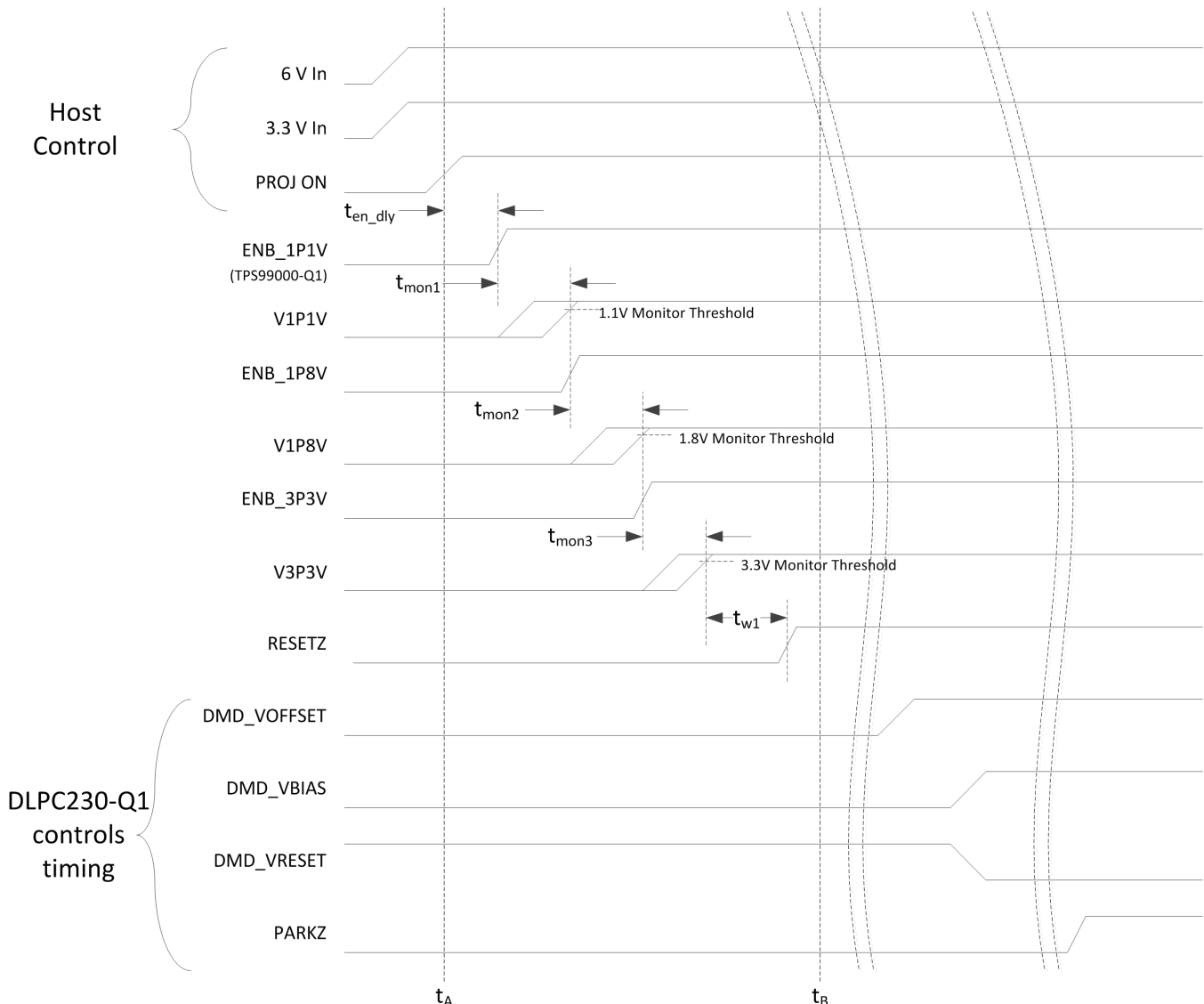
Figure 1. Power Up Timing
