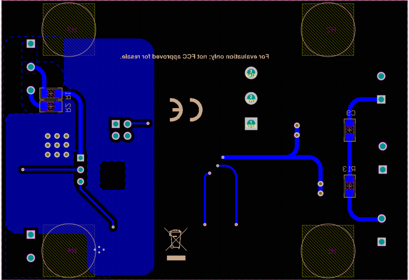
Figure 11-3. Bottom Layer
