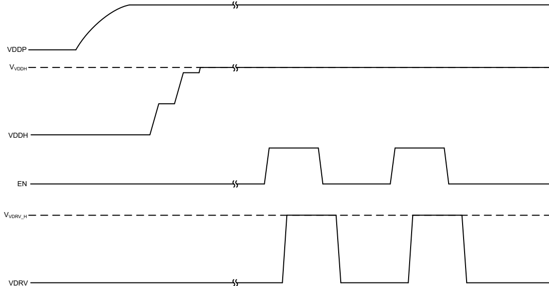
Figure 8-2. Three-Wire Mode with TPSI3050 (Standard Enable)
