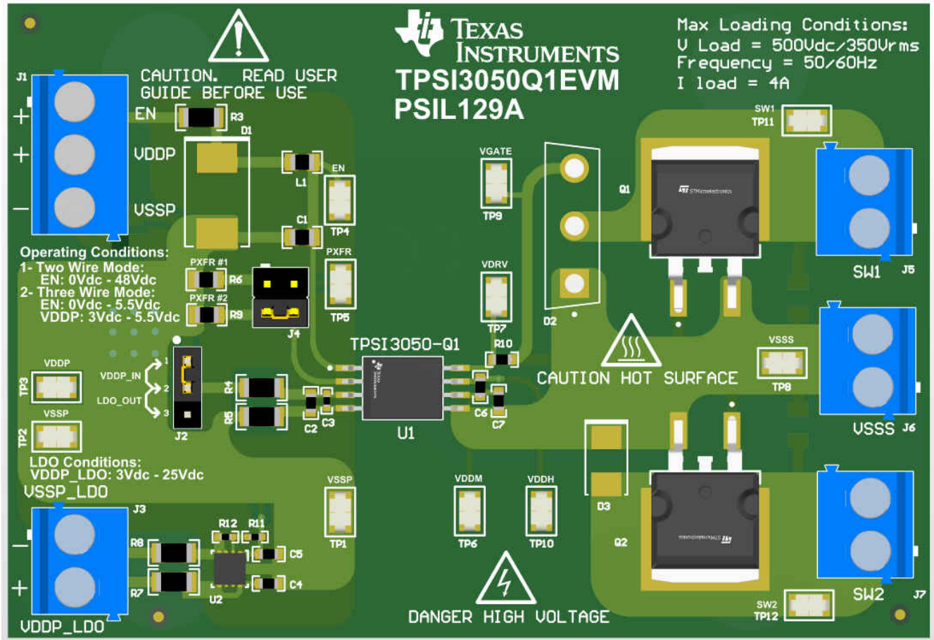
Figure 11-1. 3-D PCB View
