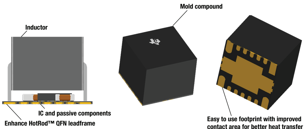
Figure 4. Power module example in the Enhanced HotRod QFN package.
