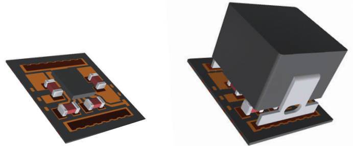
High-density layout with IC and passive components mounted on leadframe
