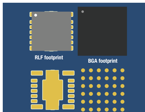
Figure 6. Thermal contact area advantage of a 5-mm-by-5.5-mm Enhanced HotRod QFN package over a 6.25-mm-by-6.25-mm BGA package.
