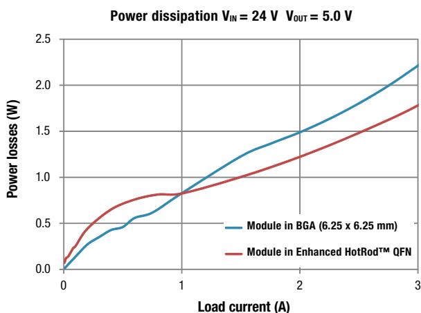
Figure 5. The power dissipation of a 6.25-mm-by-6.25-mm ball grid array (BGA) package with side-by-side inductors vs. a 5-mm-by-5.5-mm Enhanced HotRod QFN package with an over-the-top inductor.
