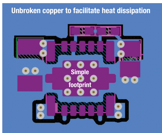
Figure 7. Easy layout with continuous copper for good thermal design.
