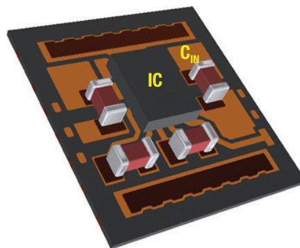
Figure 8. Placing a high-frequency bypass capacitor as close as possible to the chip minimizes the high di/dt loop area.
