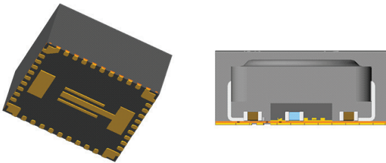
Figure 2. A power module with an inductor straddling internal module components.
