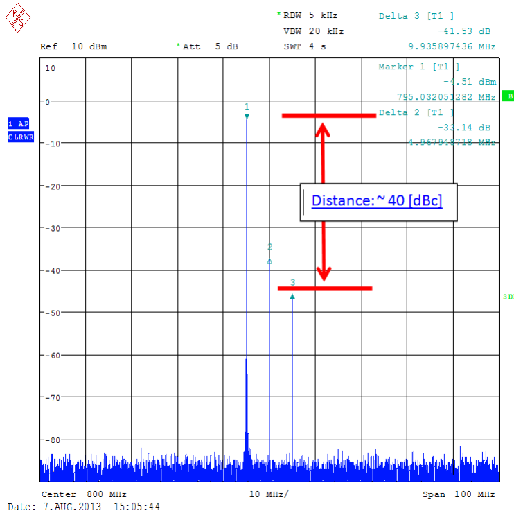
Figure 3. Example of IQ Balance Plot
