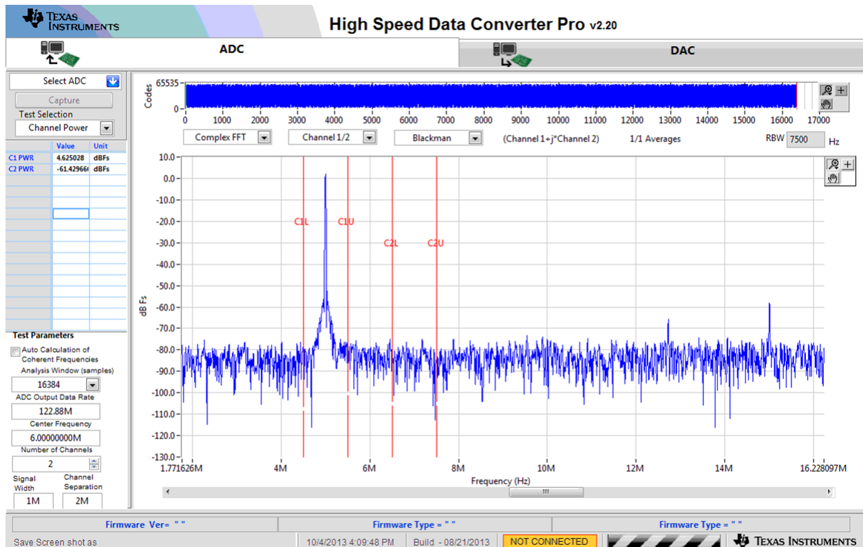
Figure 41. NSD Example
