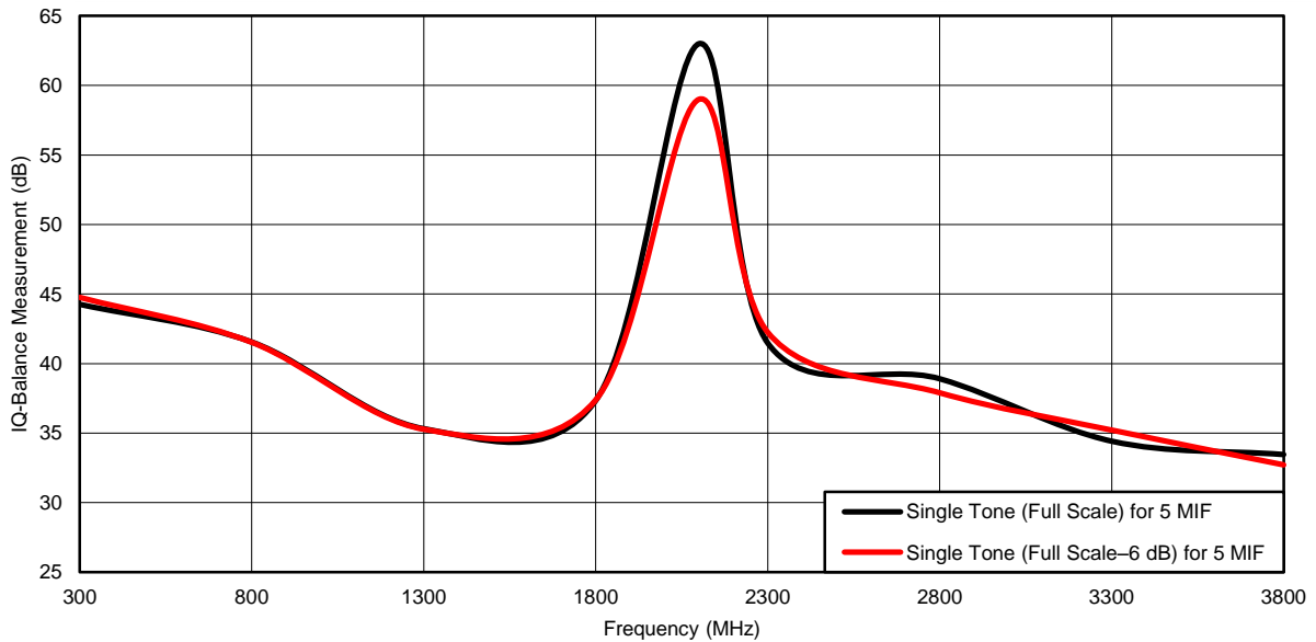
Figure 5. IQ Balance Graph for Internal LO and Bias Point of 25 \mu A
