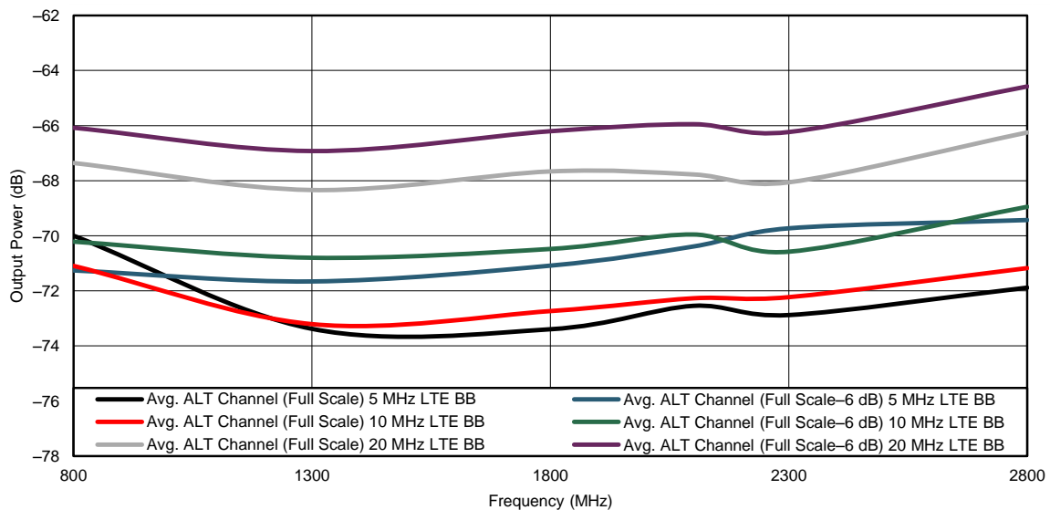
Figure 21. External LO – Alternate Channel
