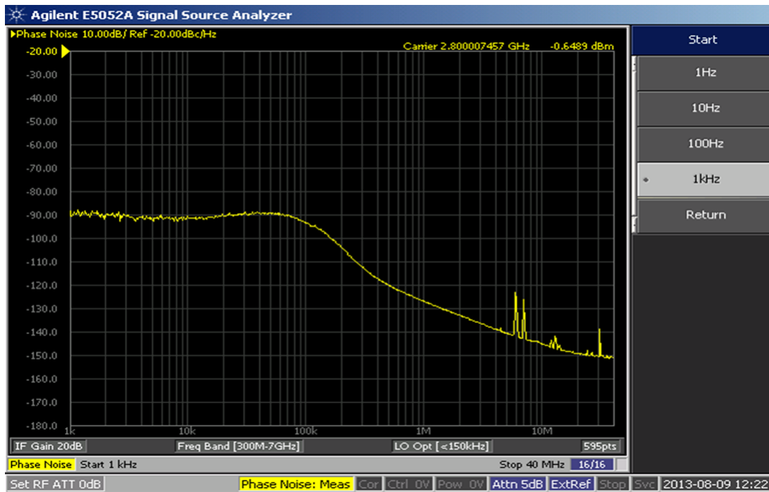
Figure 9. Phase Noise Plot – LO Carrier
