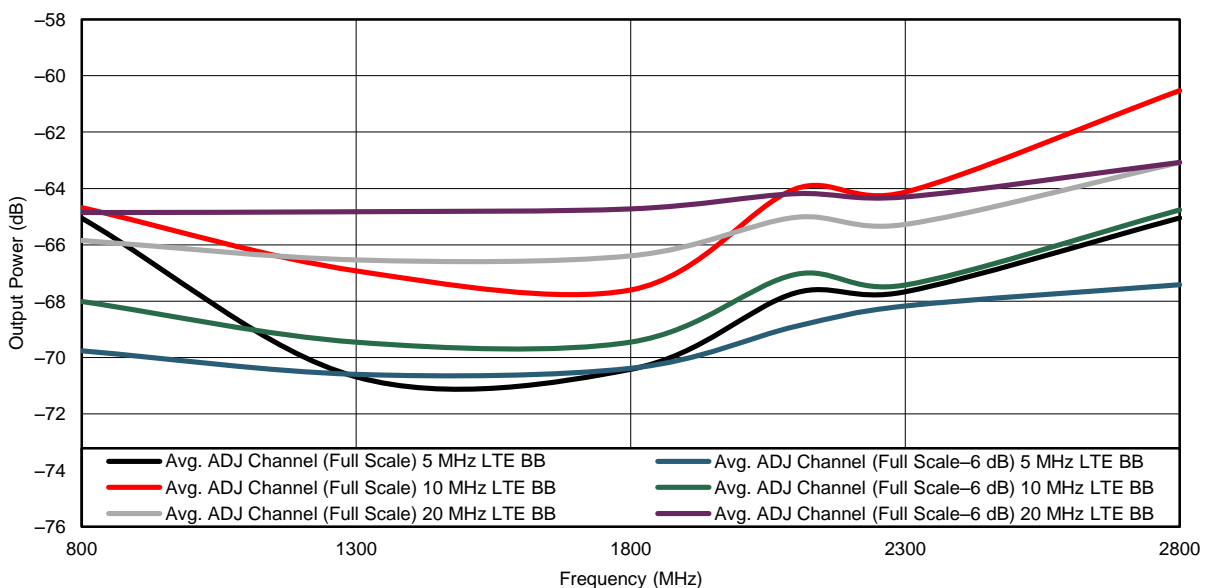
Figure 19. Adjacent Channel – External LO
