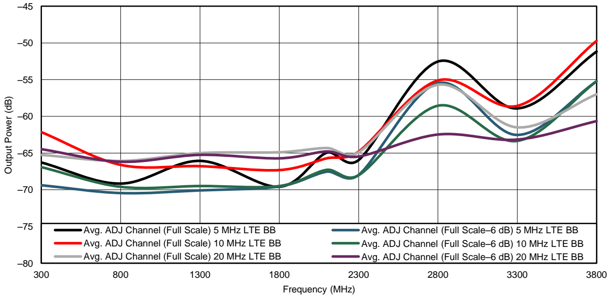
Figure 18. Adjacent Channel – Internal LO
