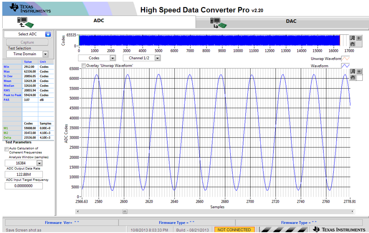
Figure 40. Backed-Off Signal
