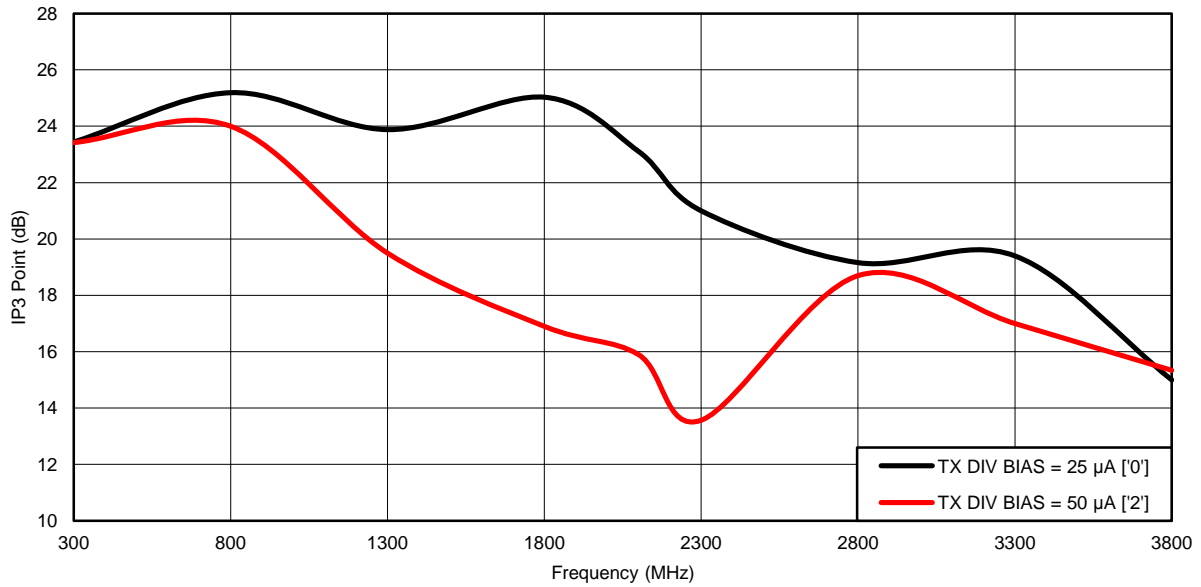
Figure 8. IP3 Plot – Internal LO
