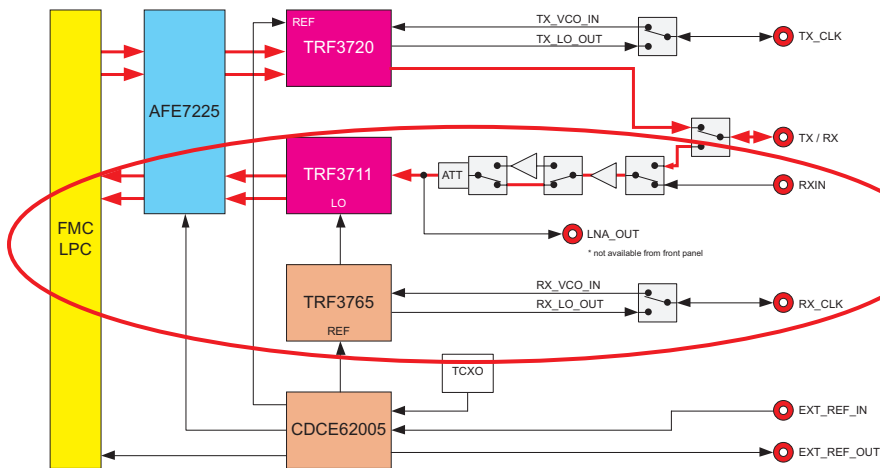
Figure 37. FMC30RF Block Diagram
