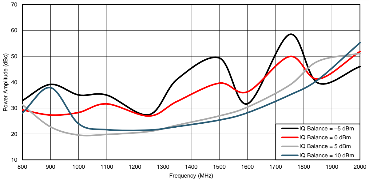
Figure 14. IQ balance, 2D Graph, Full Scaled – 1-bit IF= 10 MHz
