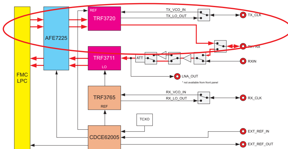
Figure 2. FMC30RF Block Diagram (TX Path Inside the Red Circle)
