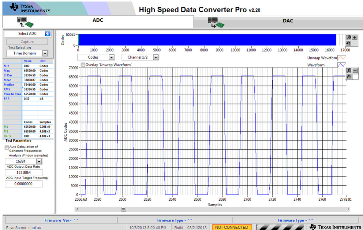
Figure 39. Saturated Signal
