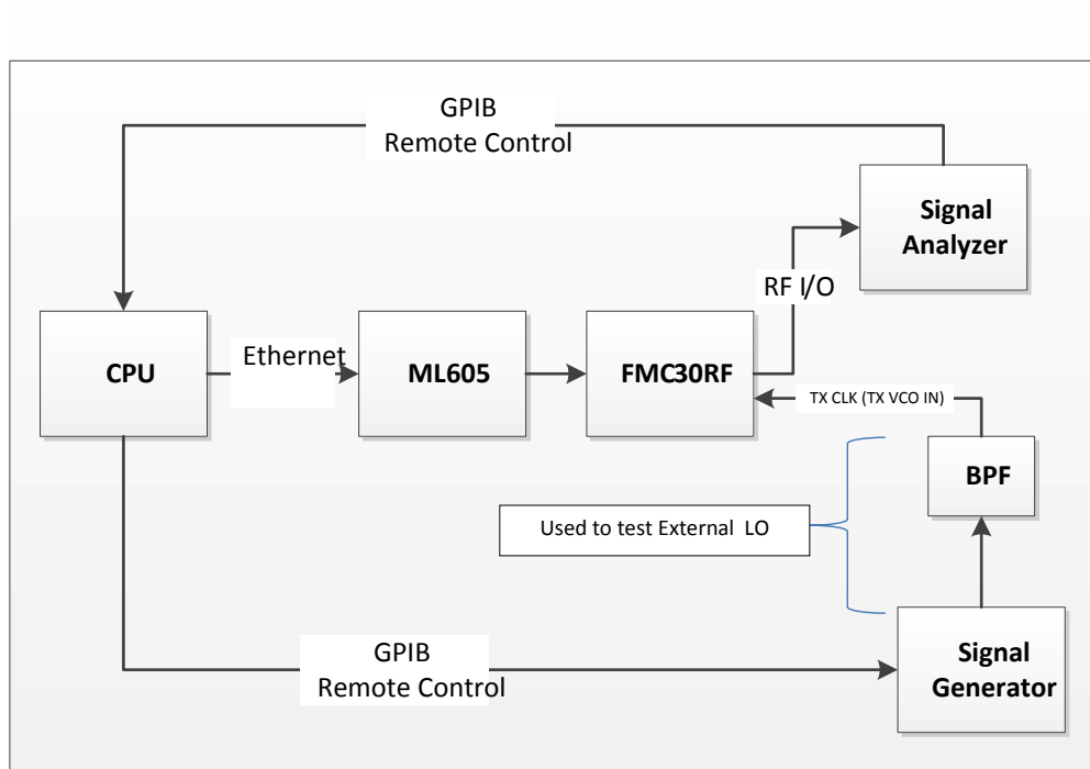
Figure 1. Block Diagram
