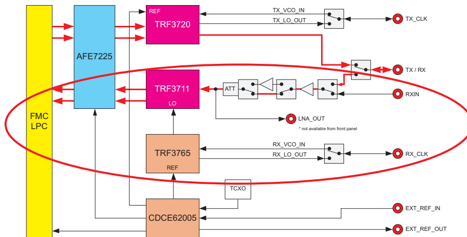
Figure 31. FMC30RF Block Diagram RX Path
