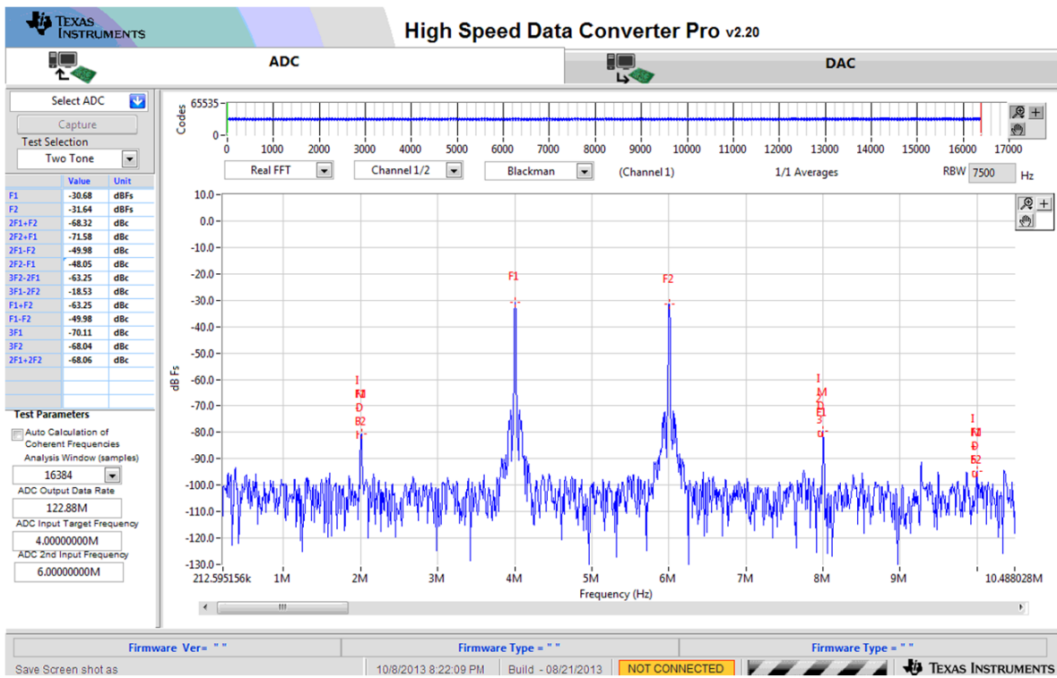
Figure 38. Two-Tone Measurement Example
