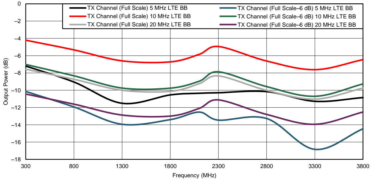
Figure 16. Internal LO – TX Channel Full Scale versus [Full Scale – 6 dB]
