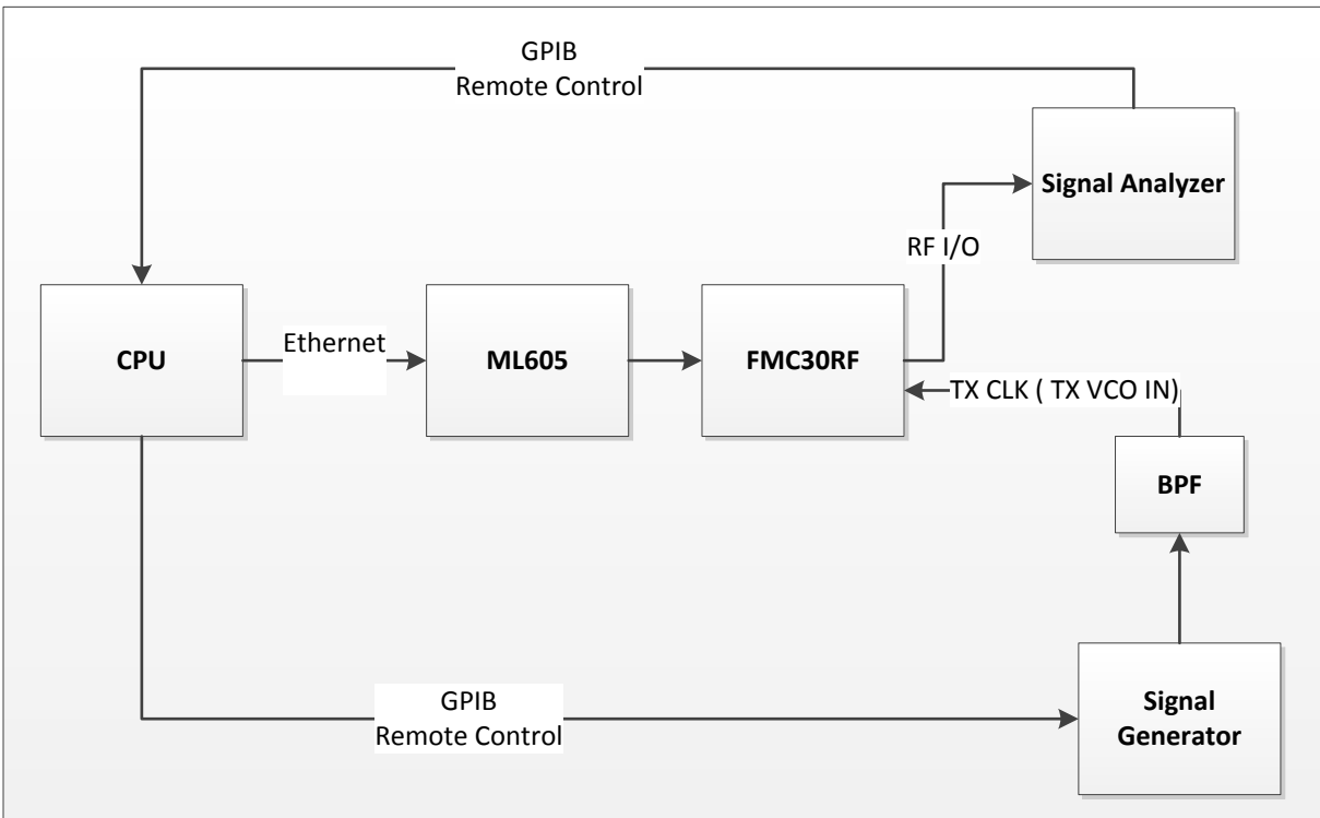
Figure 11. Block Diagram: External LO
