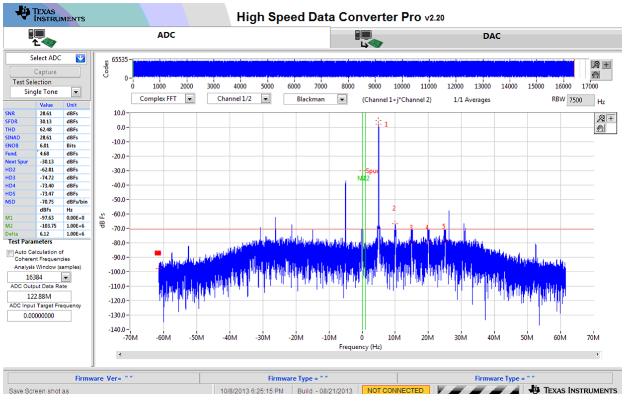
Figure 24. IQ Balance – Internal LO 5 MHz IF
