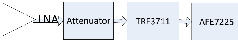
Figure 25. RX Signal Chain Block Diagram
