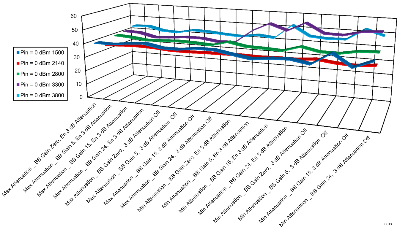
Figure 26. IQ Balance Internal LO, Pin = 0 dBm
