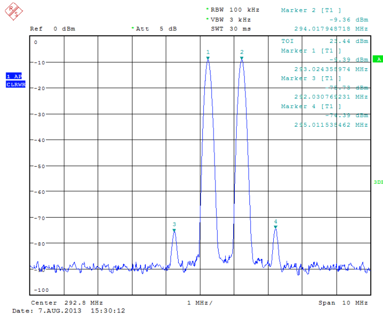
Figure 7. TX of Two Tones (Markers 1 and 2) and the IP3 Products Result (Markers 3 and 4)
