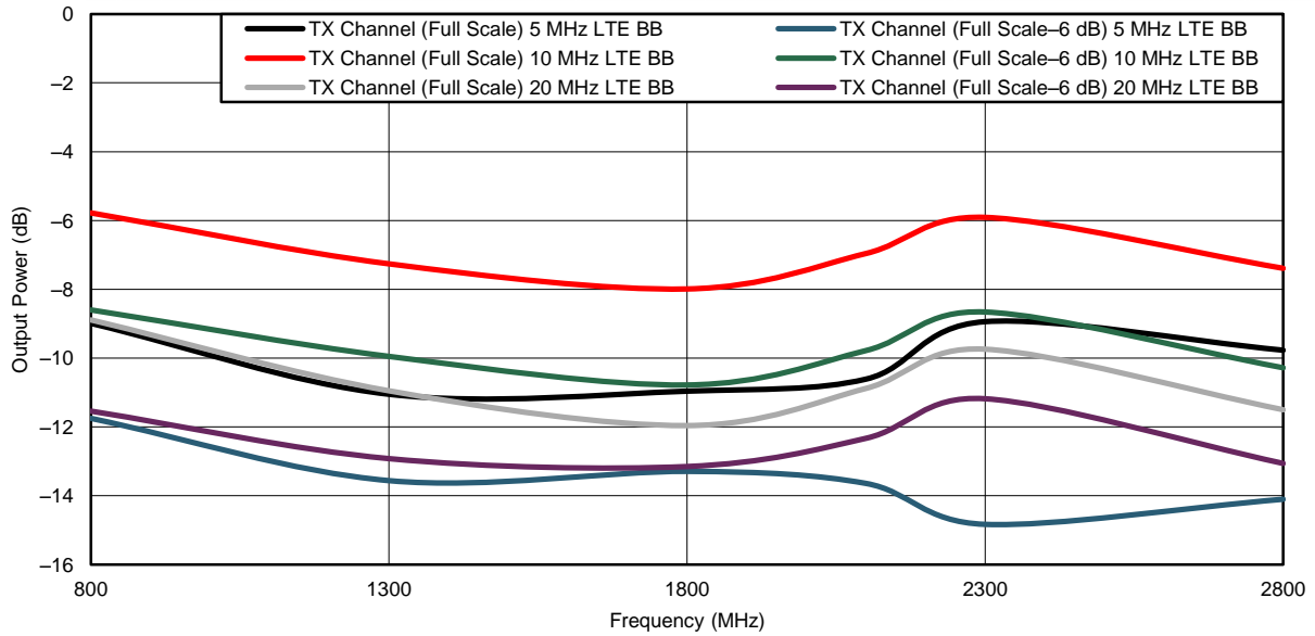
Figure 17. External LO: TX Channel Full Scale versus [Full scale – 6 dB]
