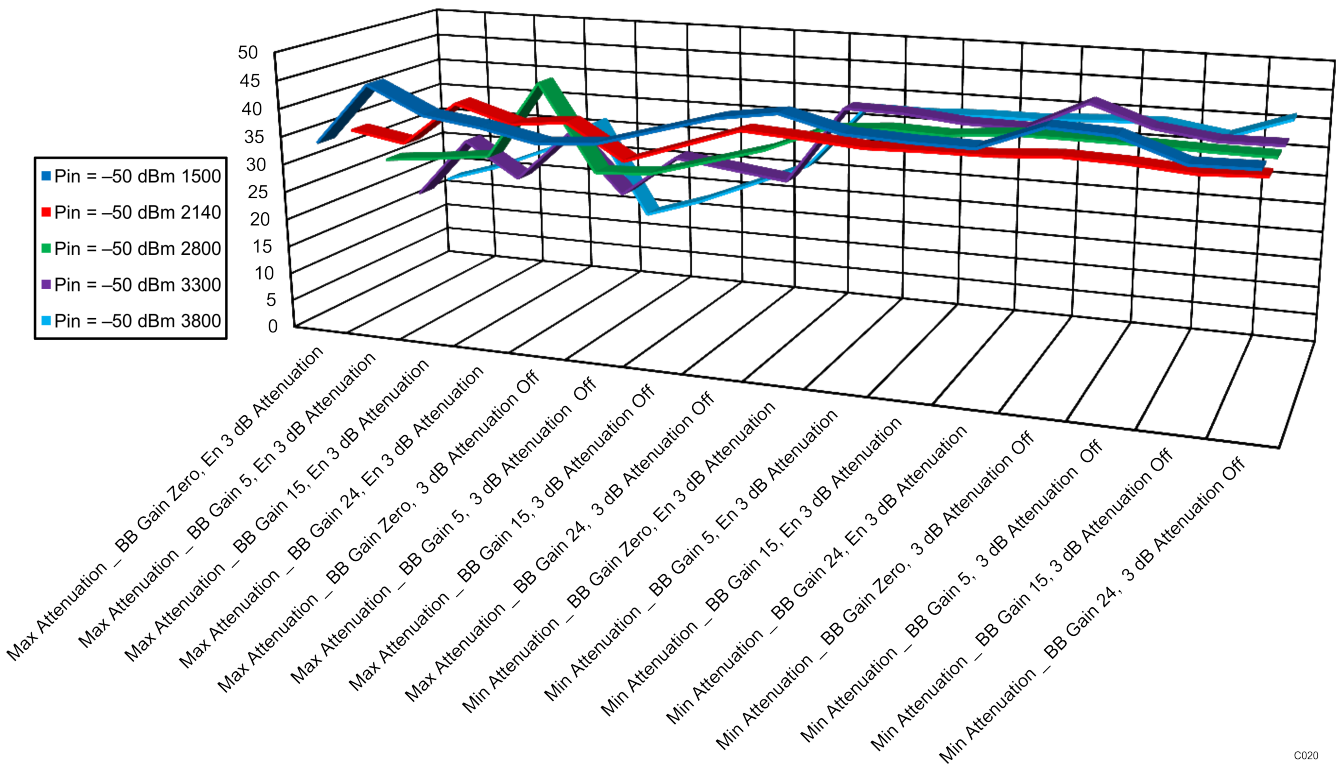
Figure 35. IQ Balance External LO, Pin = -50 dBm
