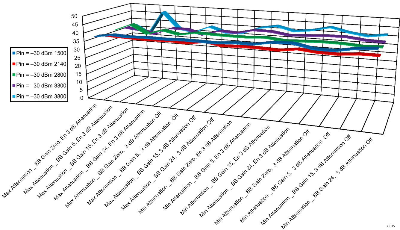
Figure 28. IQ Balance Internal LO, Pin = -30 dBm
