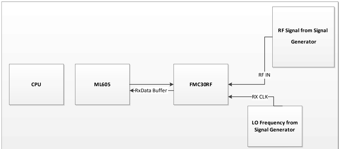
Figure 30. External LO Block Diagram
