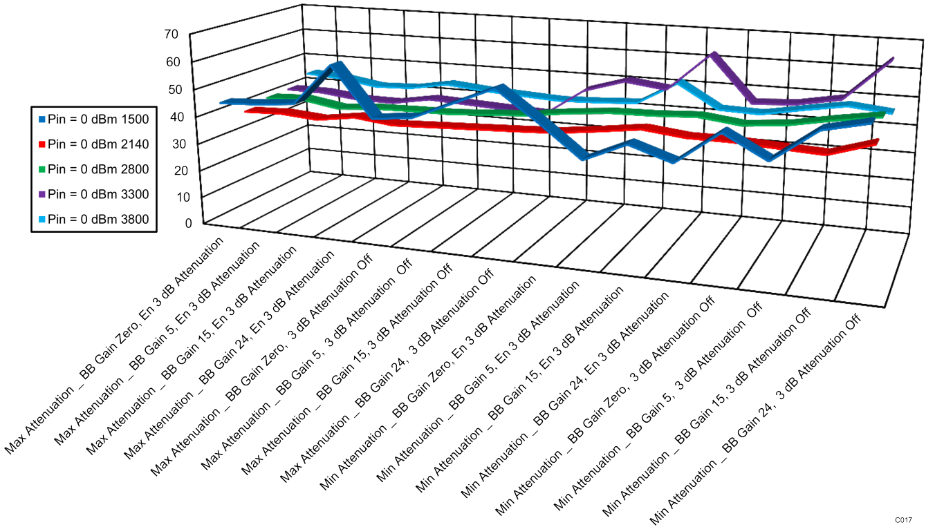
Figure 32. IQ Balance External LO, Pin = 0 dBm
