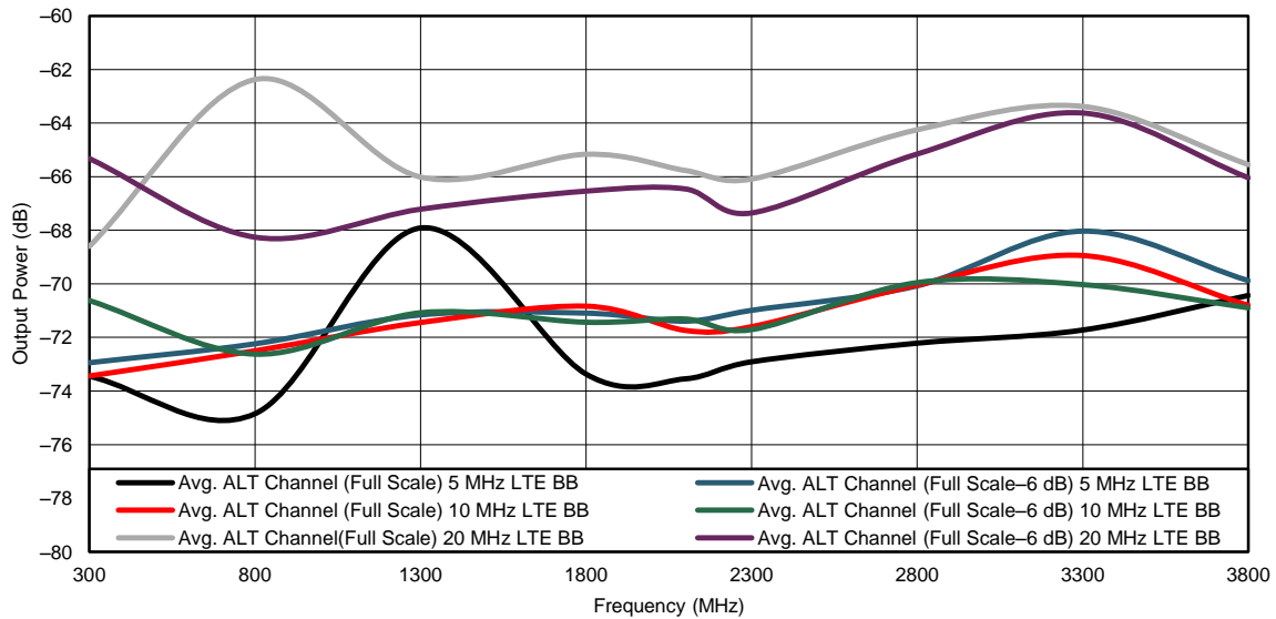
Figure 20. Internal LO: Alternate Channel
