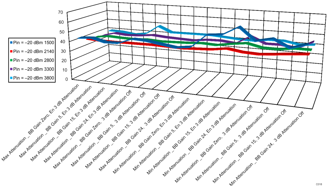
Figure 33. IQ Balance External LO, Pin = -20 dBm
