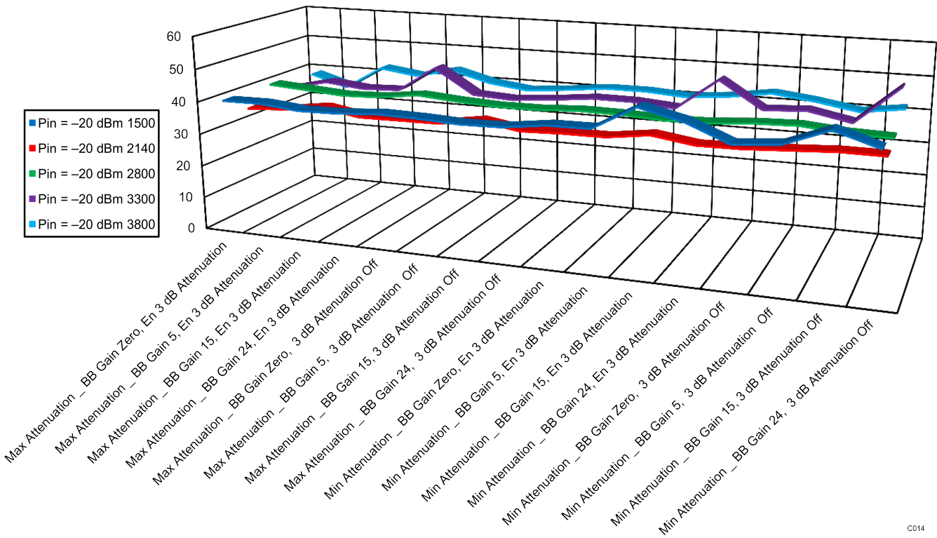
Figure 27. IQ Balance Internal LO, Pin = -20 dBm
