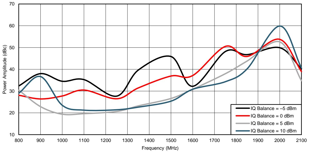
Figure 13. IQ Balance IF = 10 MHz Full Scaled Signal
