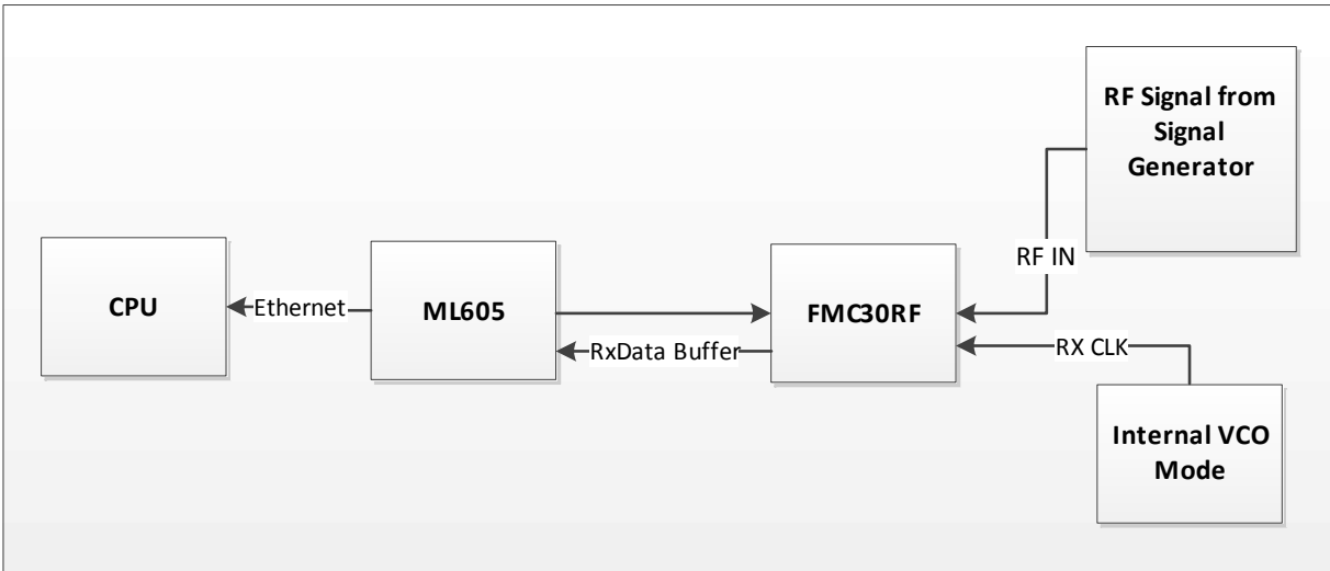
Figure 22. Block Diagram Internal LO
