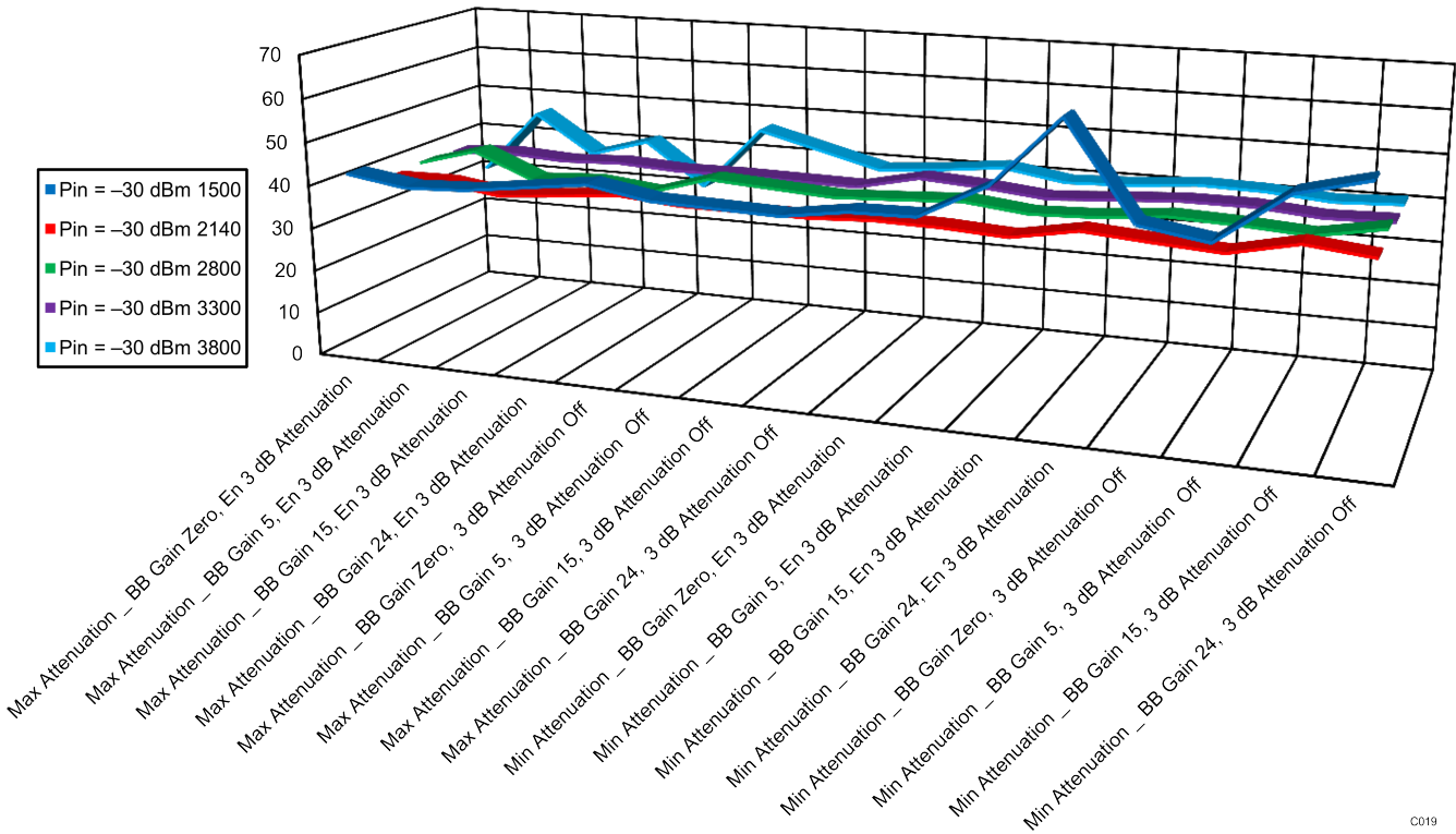
Figure 34. IQ Balance External LO, Pin = -30 dBm
