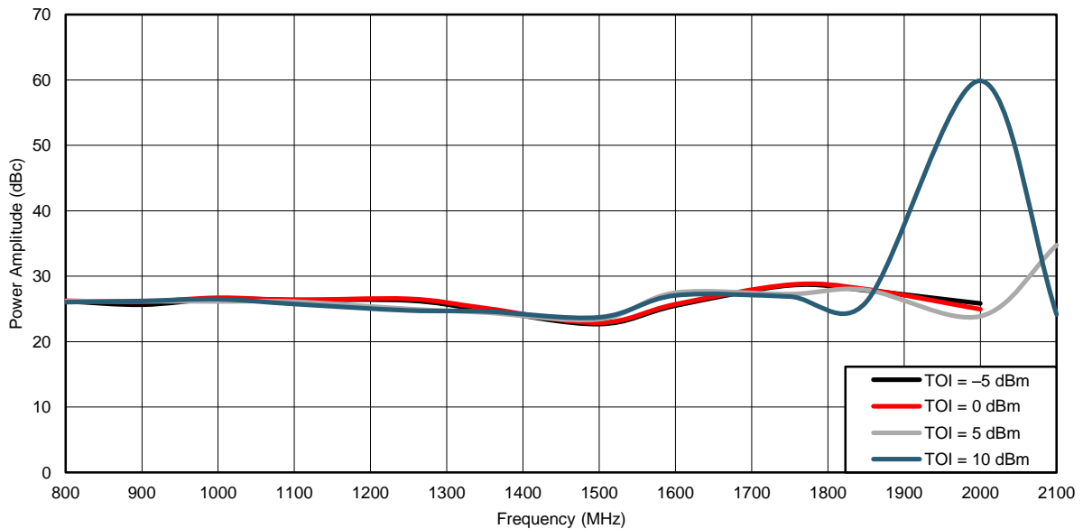
Figure 15. TOI – External LO
