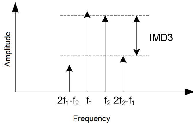
Figure 4. Frequency versus Amplitude for IMD3 Products
