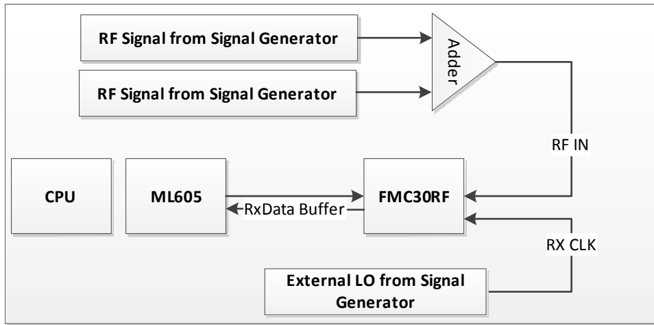
Figure 36. Block Diagram Internal / External LO
