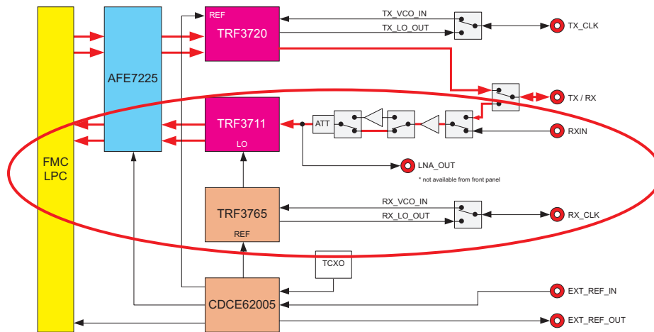
Figure 23. FMC30RF Block Diagram
