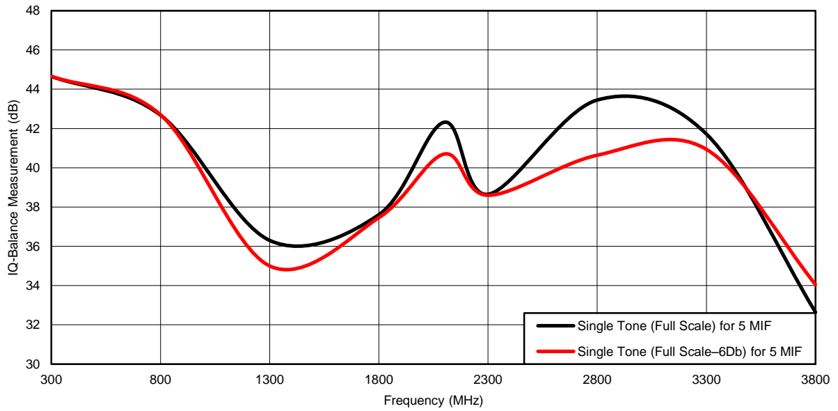
Figure 6. IQ Balance Graph for Internal LO and Bias Point of 50 \mu A
