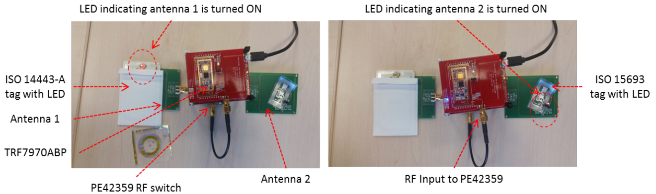
Figure 9. Prototype of TRF7970ABP + PE42359 RF Switch Demonstration
