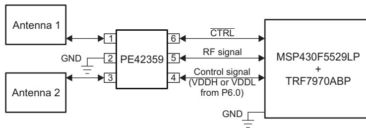
Figure 6. Complementary-Pin Control Method
