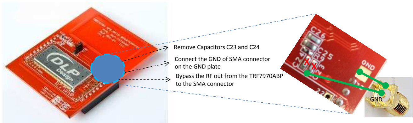
Figure 3. TRF7970A BP Modifications
