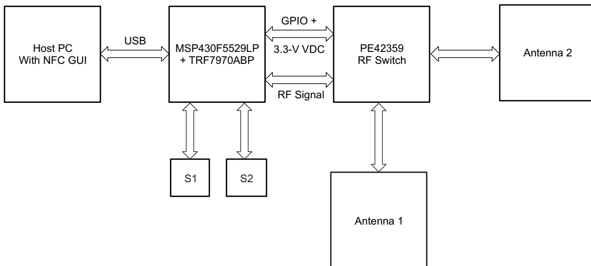
Figure 1. Block Diagram of Reader Antenna Multiplexing Demo
