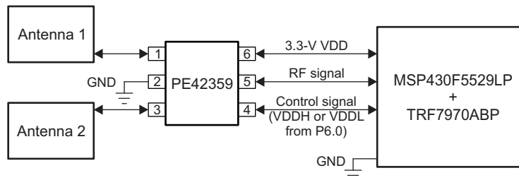
Figure 5. Single-Pin Control Method
