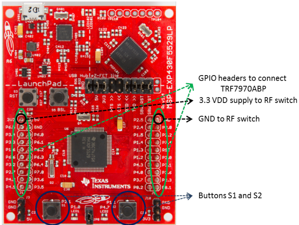
Figure 2. MSP430F5529 LaunchPad Development Kit
