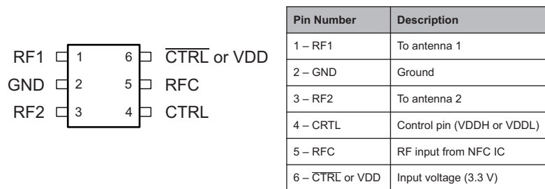
Figure 4. PE42359 RF Switch Pin Configuration and Description
