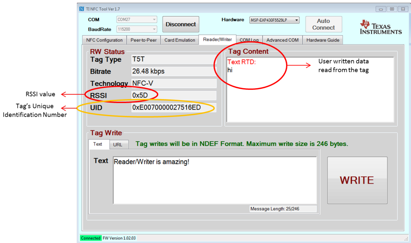
Figure 10. NFC Tool GUI in Reader/Writer Mode
