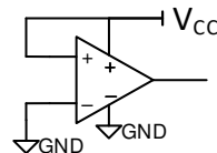
Wrong: No Resistors
