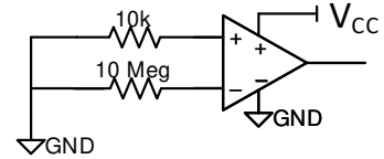
Ok: V_{OL} ( I_{IB} Biased)
