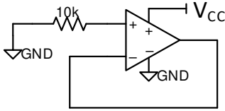
Ok: Soft V_{OL}
