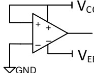
Figure 7-4. Potentially Harmful Connection Practices for Single and Dual Supplies
