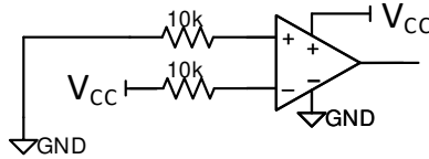
Ok: V_{OL} Full V_{ID} ( V_{CC} < 24\text{ V} )
