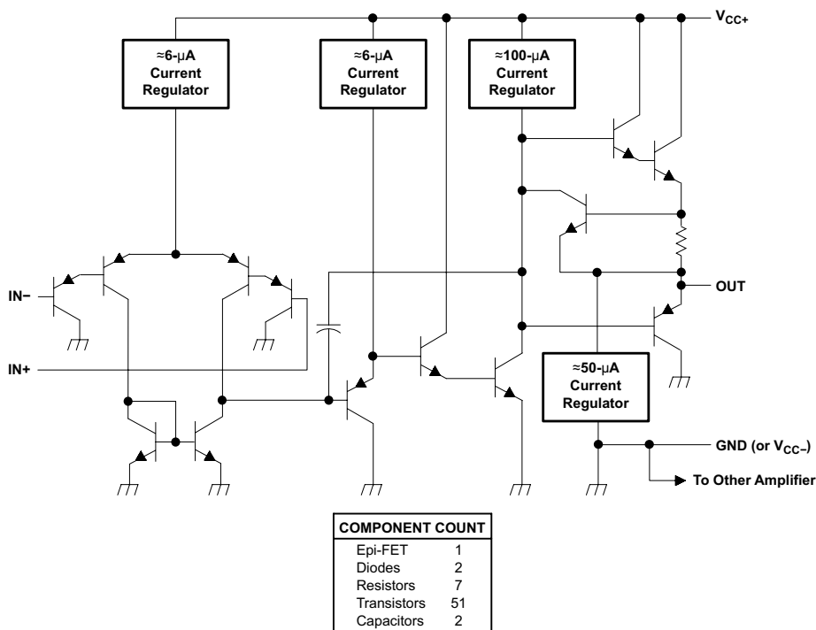
Figure 1-1. Device Schematic from Data Sheet
