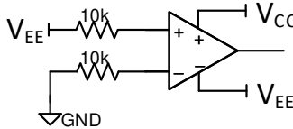
Figure 7-2. Acceptable Connection Practices for Single and Dual Supplies
