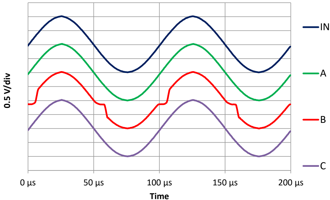
Figure 4-6. LM324 Crossover Test Waveforms
