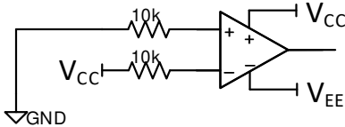
Figure 7-2. Acceptable Connection Practices for Single and Dual Supplies
