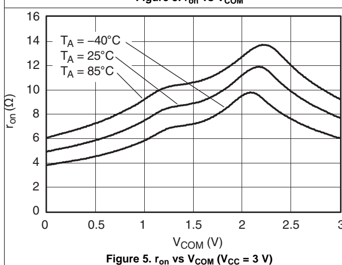
Figure 5. r_{on} vs V_{COM} ( V_{CC} = 3 V)
