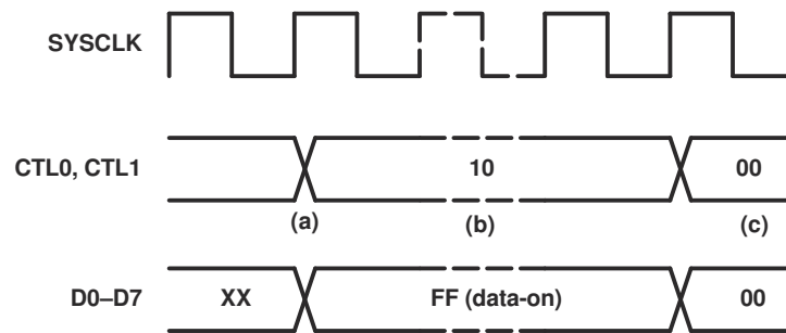
Figure 12-5. Null Packet Reception Timing
