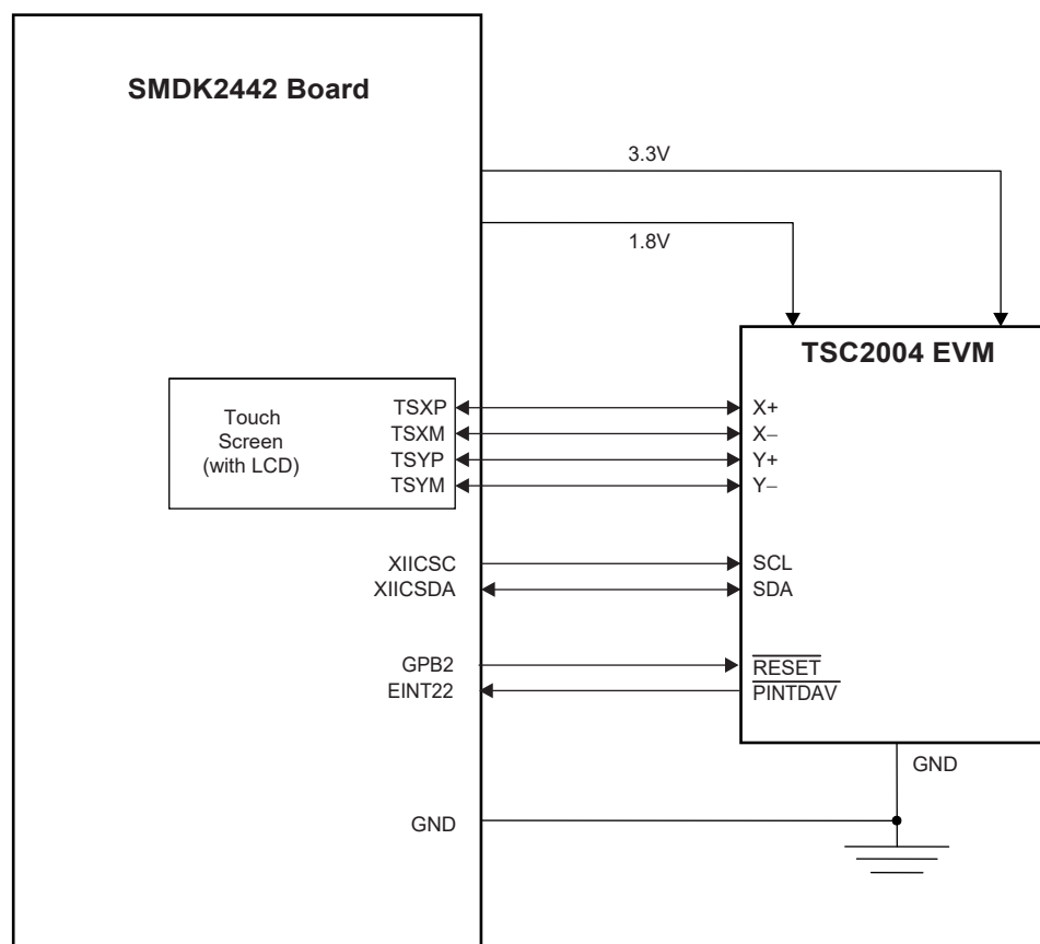
Figure 1. TSC2004 Connection to SC32442 Application Processor
