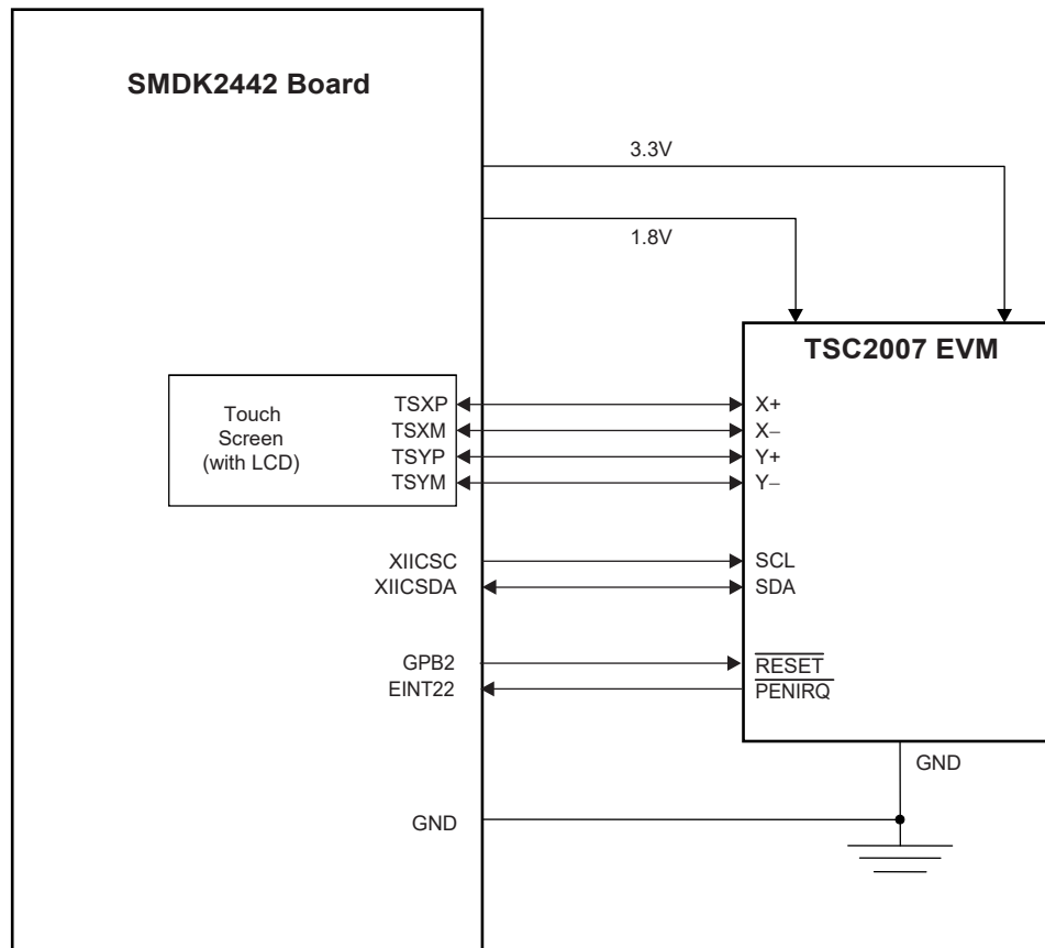
Figure 1. TSC2007 Connection to SC32442 Application Processor
