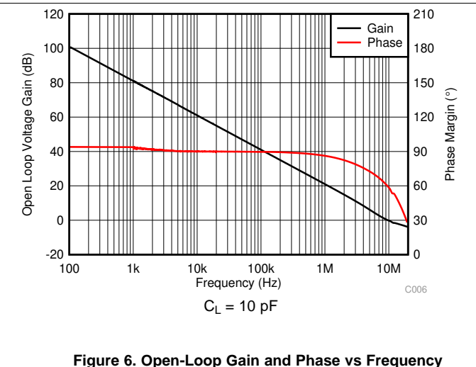
Figure 6. Open-Loop Gain and Phase vs Frequency
