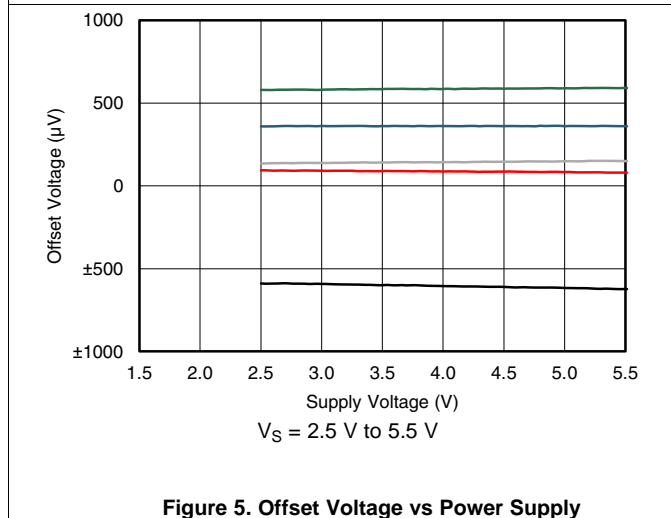
Figure 5. Offset Voltage vs Power Supply
