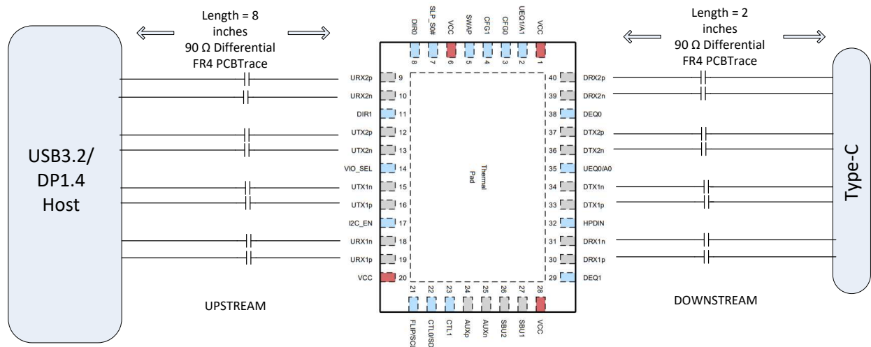
Figure 1. System Trace Length Example
