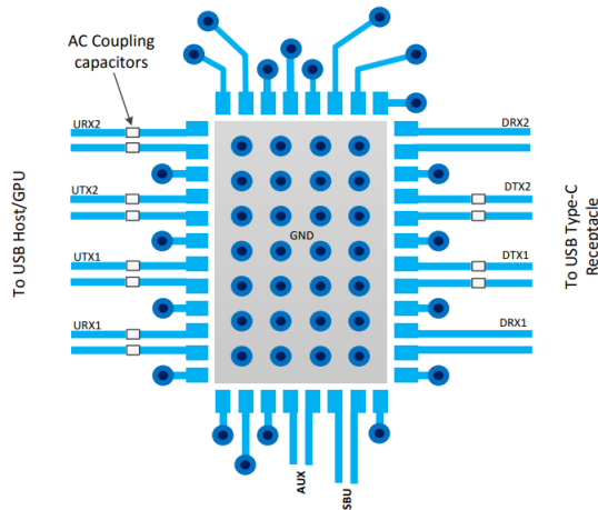
Figure 3. AC-Coupling Capacitor Placement
