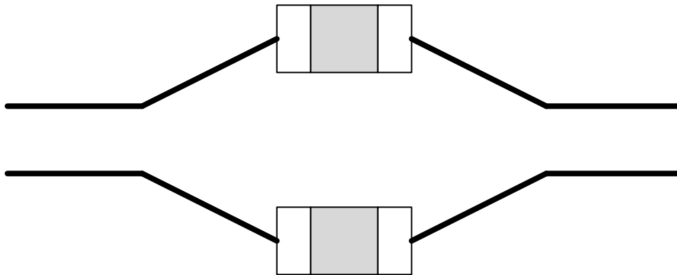
Figure 4. AC-Coupling Capacitor Layout Symmetry Example
