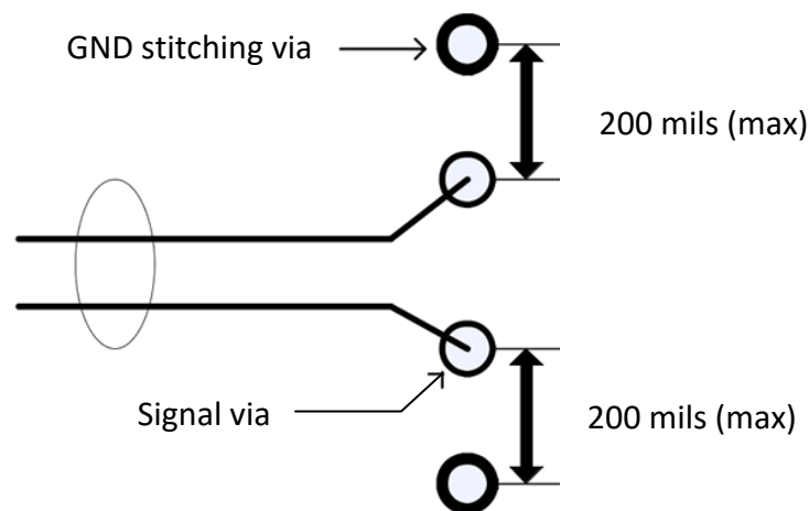
Figure 2. GND Stitching Via Example
