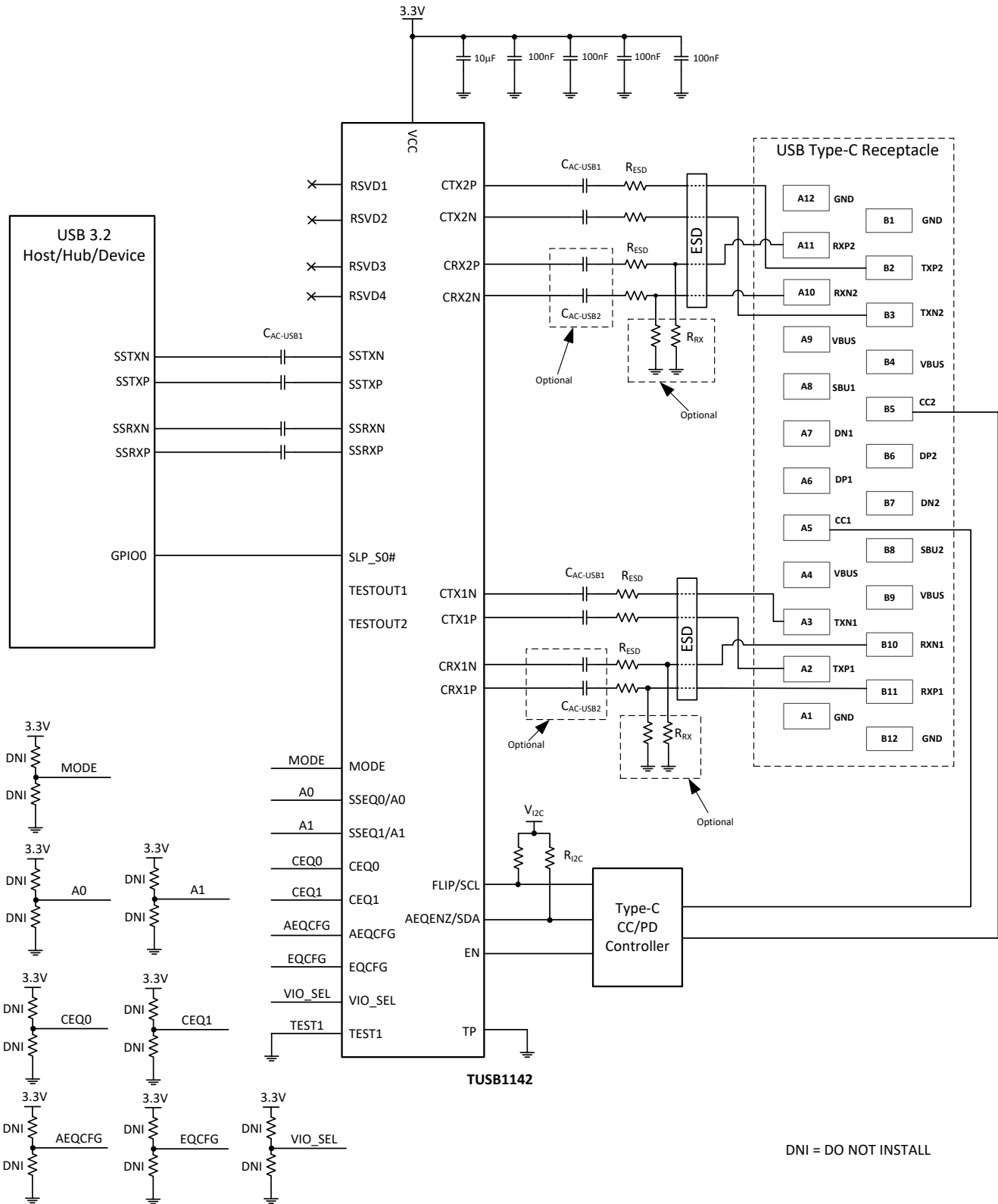
Figure 11-1. Application Circuit
