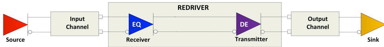
Figure 6. Example of a redriver concept.
