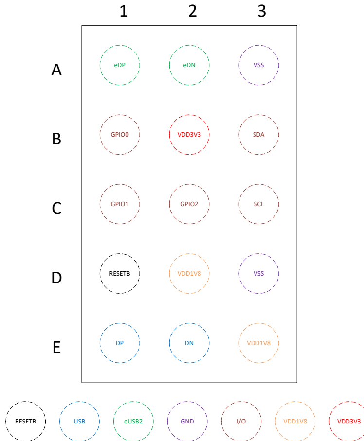
Figure 6-1. TUSB2E11 YCG Package, 15-Pin DSBGA (Top View)
