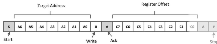
Figure 8-9. I 2 C Write Without Data
