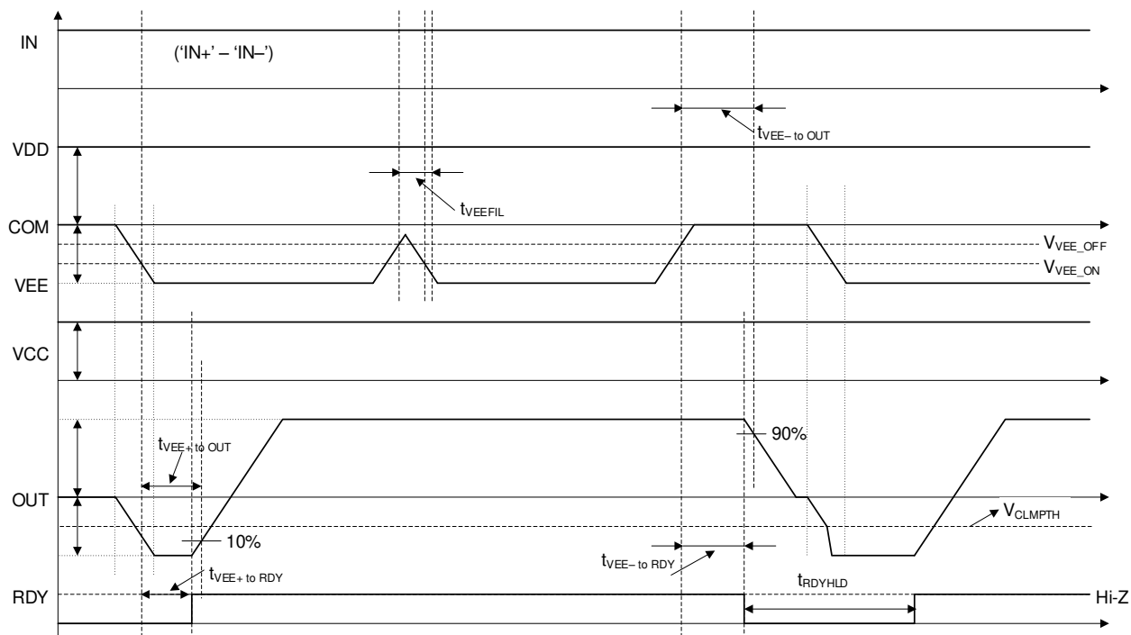
Figure 7-10. VEE UVLO Protection Timing Diagram
