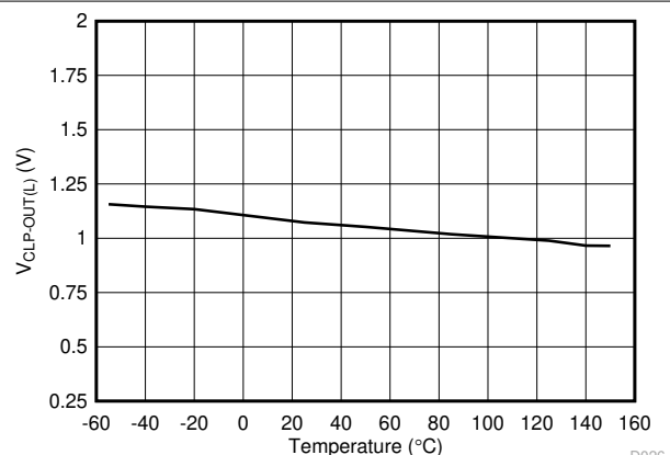
Figure 6-20. V_{CLP-OUT(L)} Short Circuit Clamping Voltage vs Temperature
