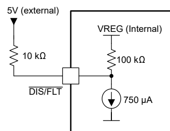
Figure 7-17. External Pullup for 5-V Supply
