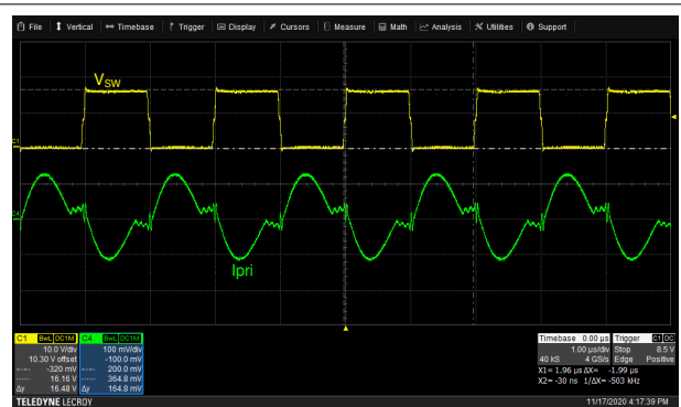
Figure 8-11. Switch-node Voltage (yellow) and Current (Primary side, 0.2V/A) at Full Load
