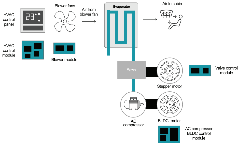
Figure 5. The heat pump system.
