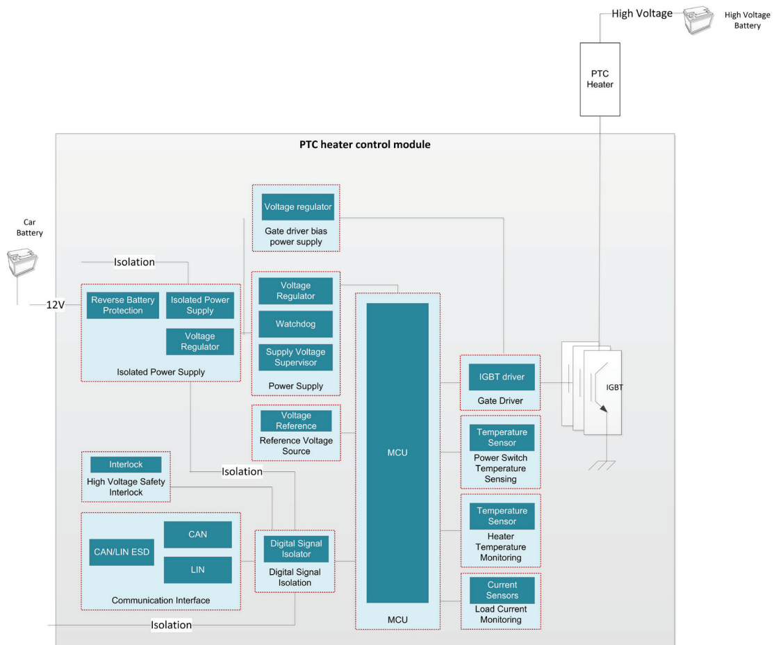
Figure 4. Block diagram of a high-voltage PTC heater control module.
