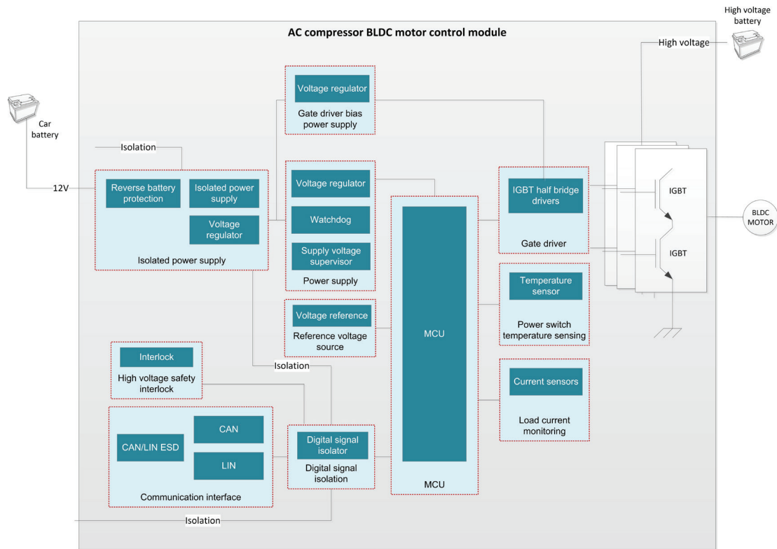
Figure 3. Block diagram of a high-voltage AC compressor BLDC motor control module.
