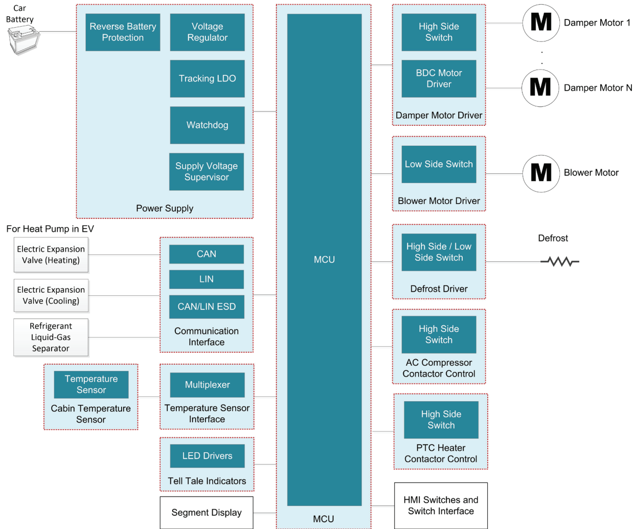
Figure 7. An HVAC control module.
