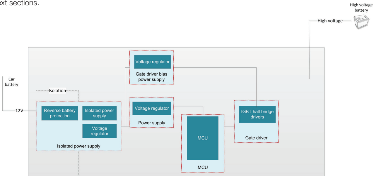
Figure 8. Powering the circuits in the control module from the 12-V rail.
