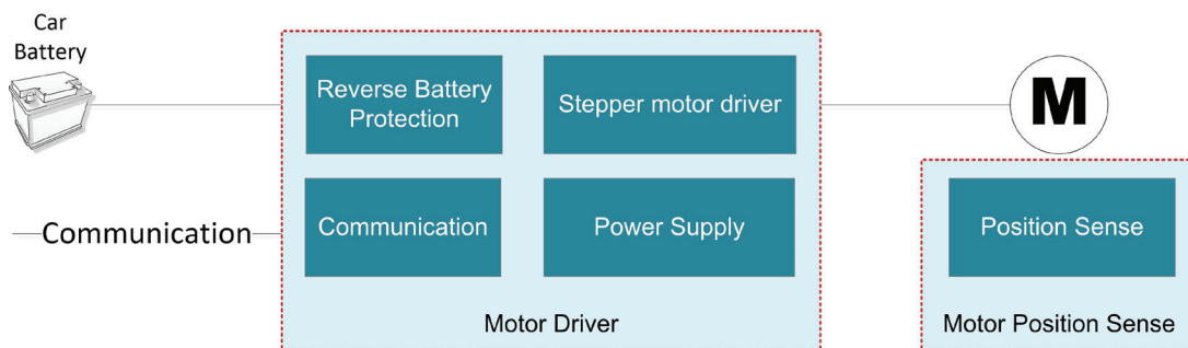
Figure 6. Block diagram of a stepper motor driver.
