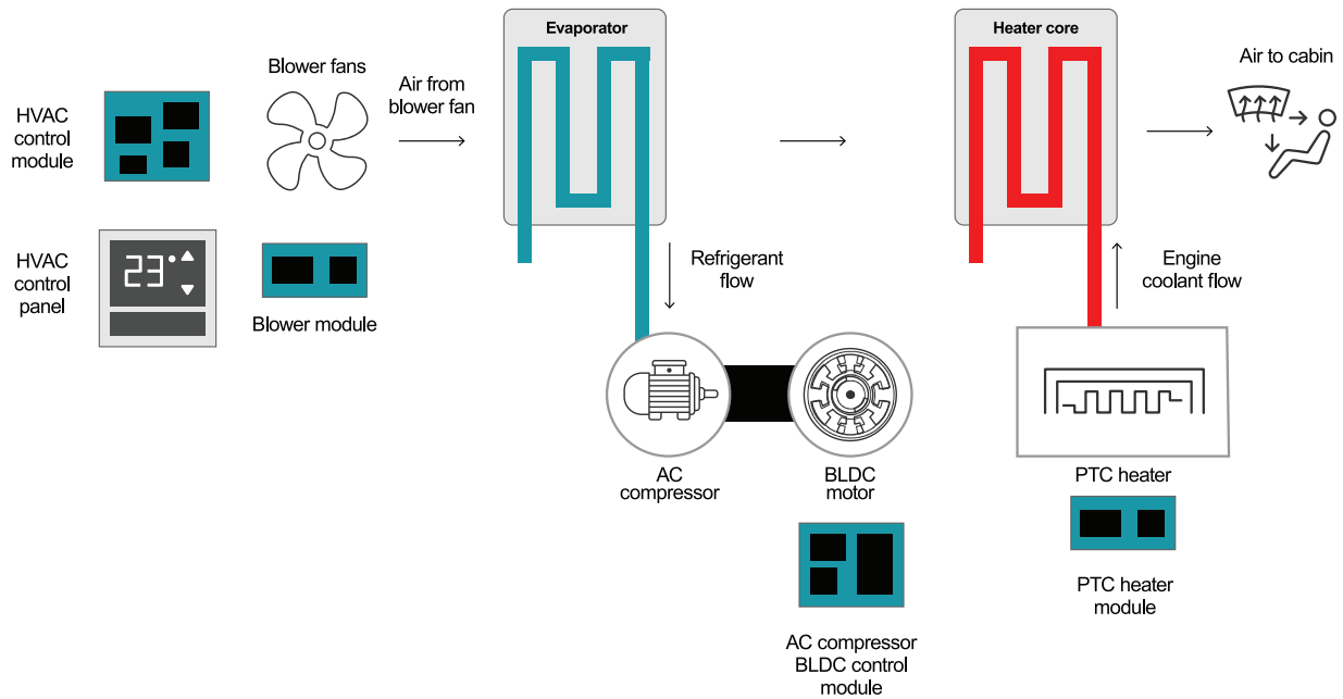
Figure 2. The heating and cooling system in a HEV/EV.
