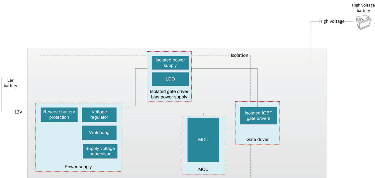
Figure 9. Powering the circuits in the control module from the 12-V rail.
