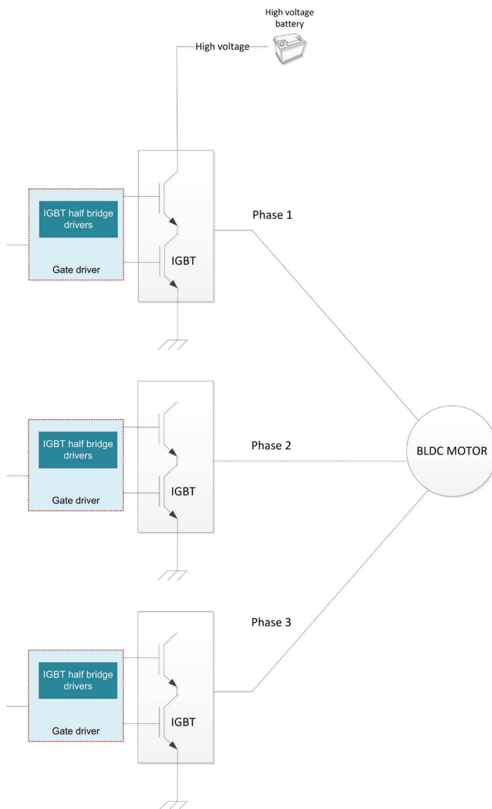
Figure 10. Driving the inverter stage with three half-bridge gate drivers.
