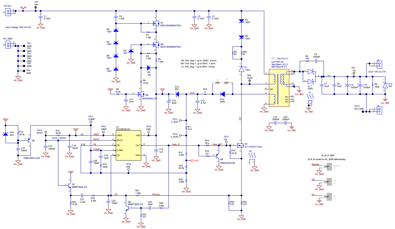
Figure 3-1. UCC28C56EVM-066 Schematic.
