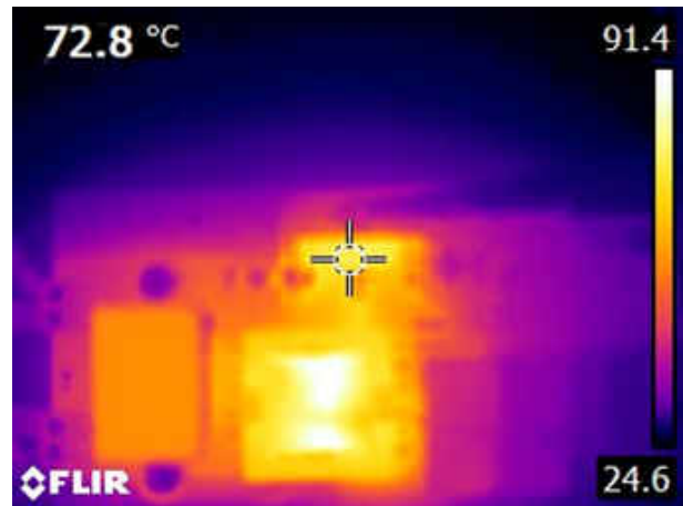
Figure 5-44. MOSFET temperature is 72.8°C
