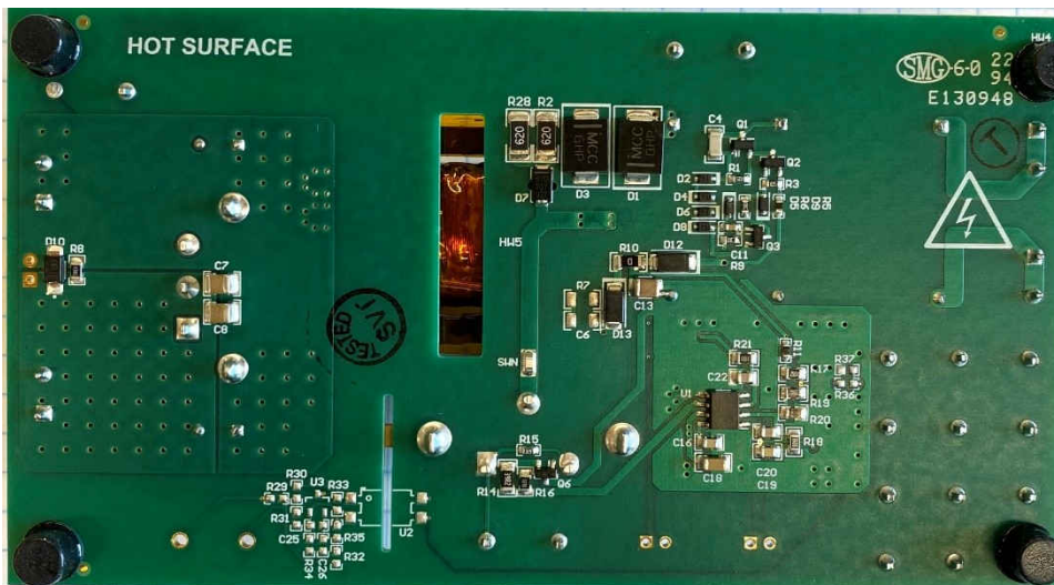
Figure 2-2. UCC28C56EVM-066, HVP066E2, Bottom View
