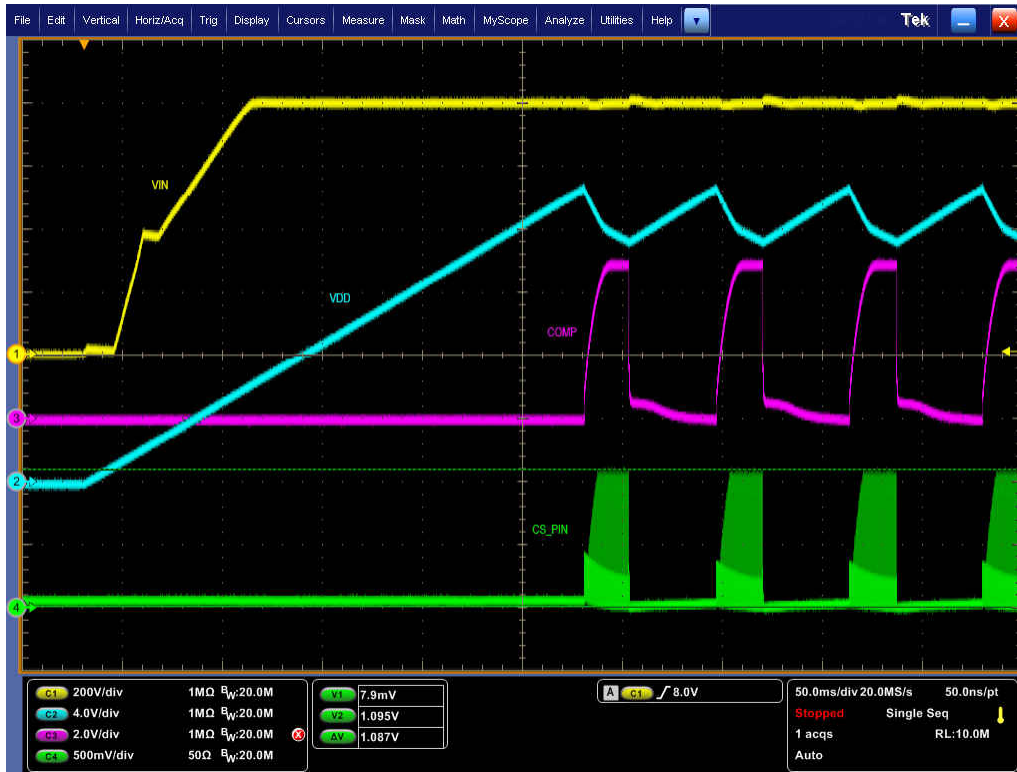
Figure 5-29. 800 VIN, Startup with output shorted to ground
