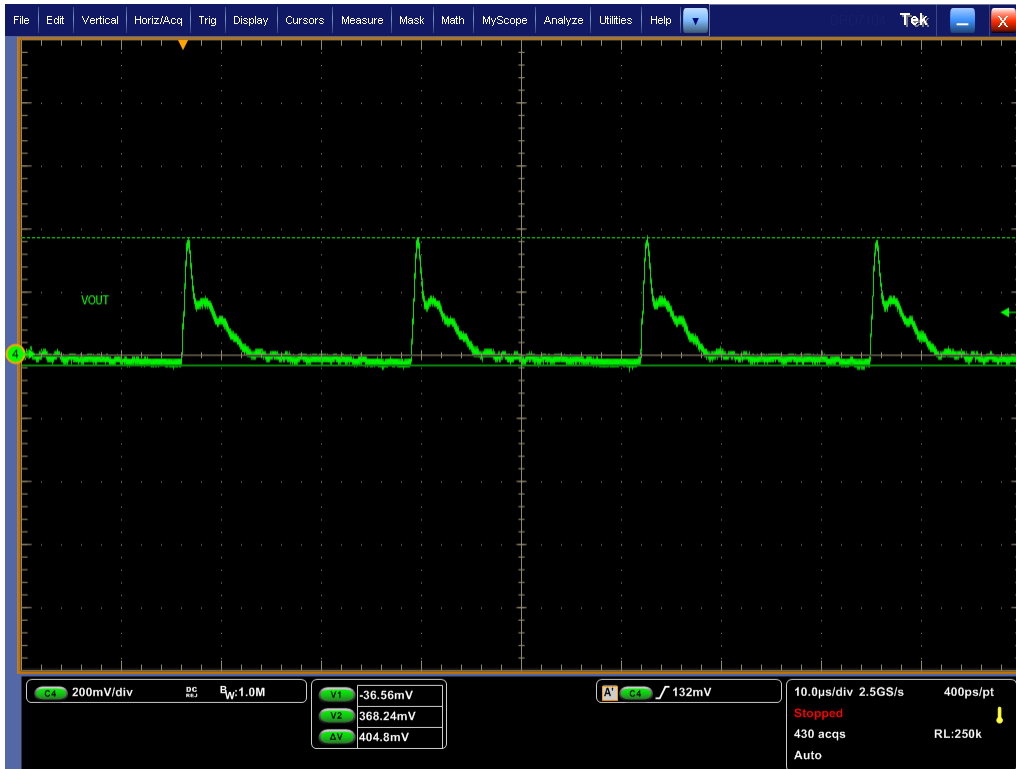
Figure 5-18. Output Voltage Ripple: VIN = 1000 V, Load = 2.7 A
