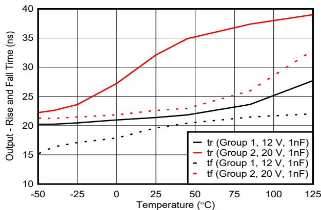
Group 1: UCC28C50-Q1 to UCC28C55-Q1 Group 2: UCC28C56H-Q1 to UCC28C59-Q1
