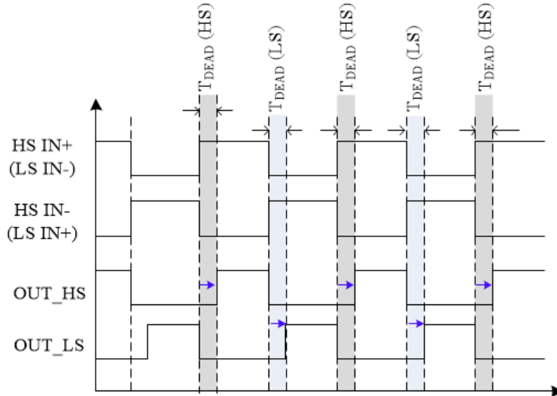
Figure 7-30. Timing scheme of implementation of STP function.
