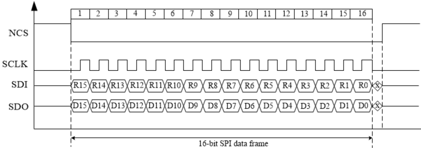
Figure 7-44. 16-bit of SPI data frame.
