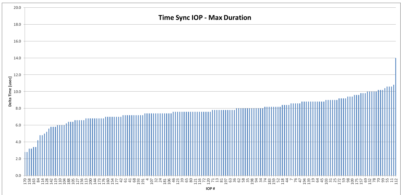
Figure 11. IOP – Max Delta Time Measured Between Two Devices for all APs
