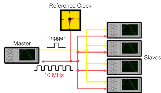
Figure 2. Synchronizing Machines
