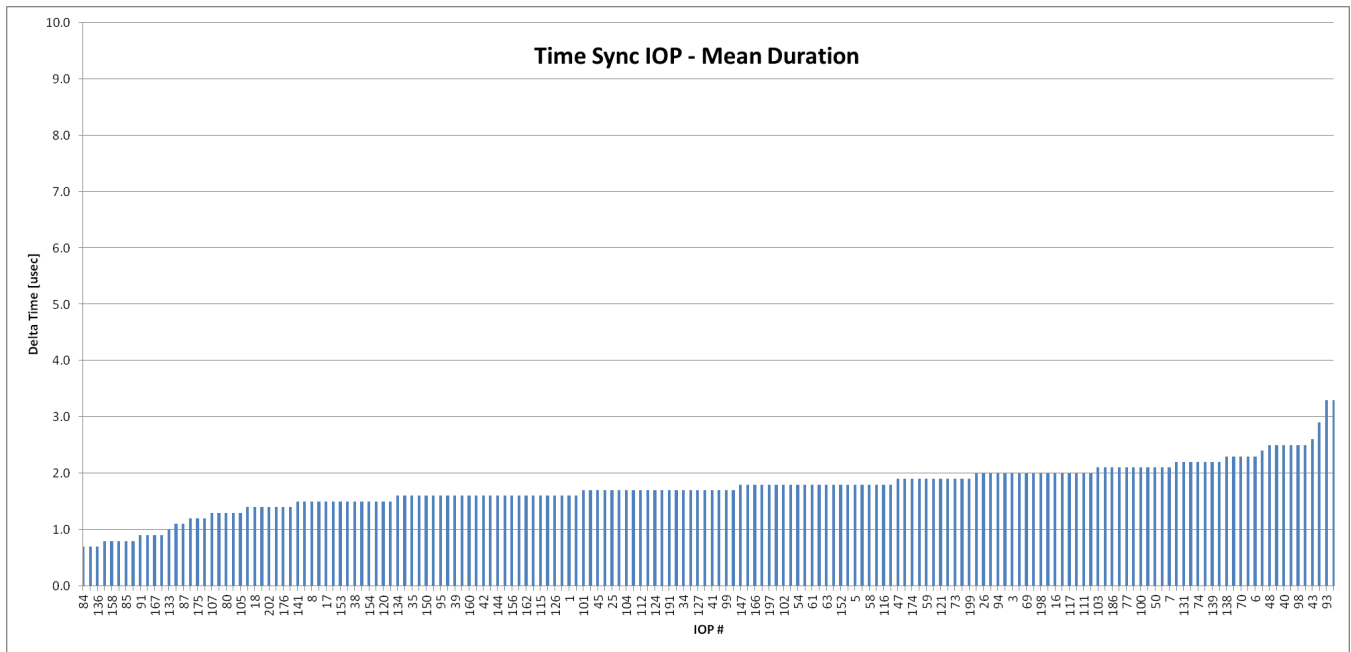
Figure 9. IOP – Mean Delta Time Between Two Devices for all APs
