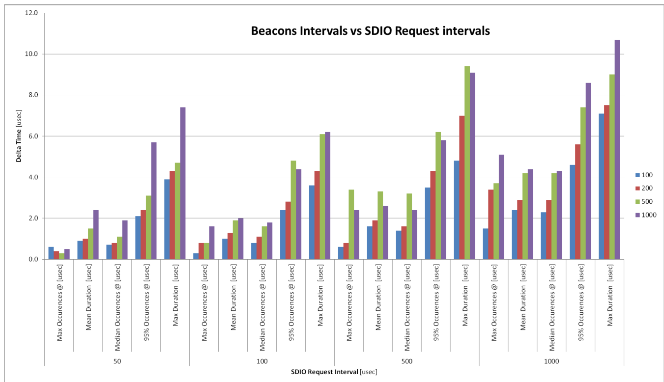
Figure 4. Beacons Intervals vs SDIO Request Intervals
