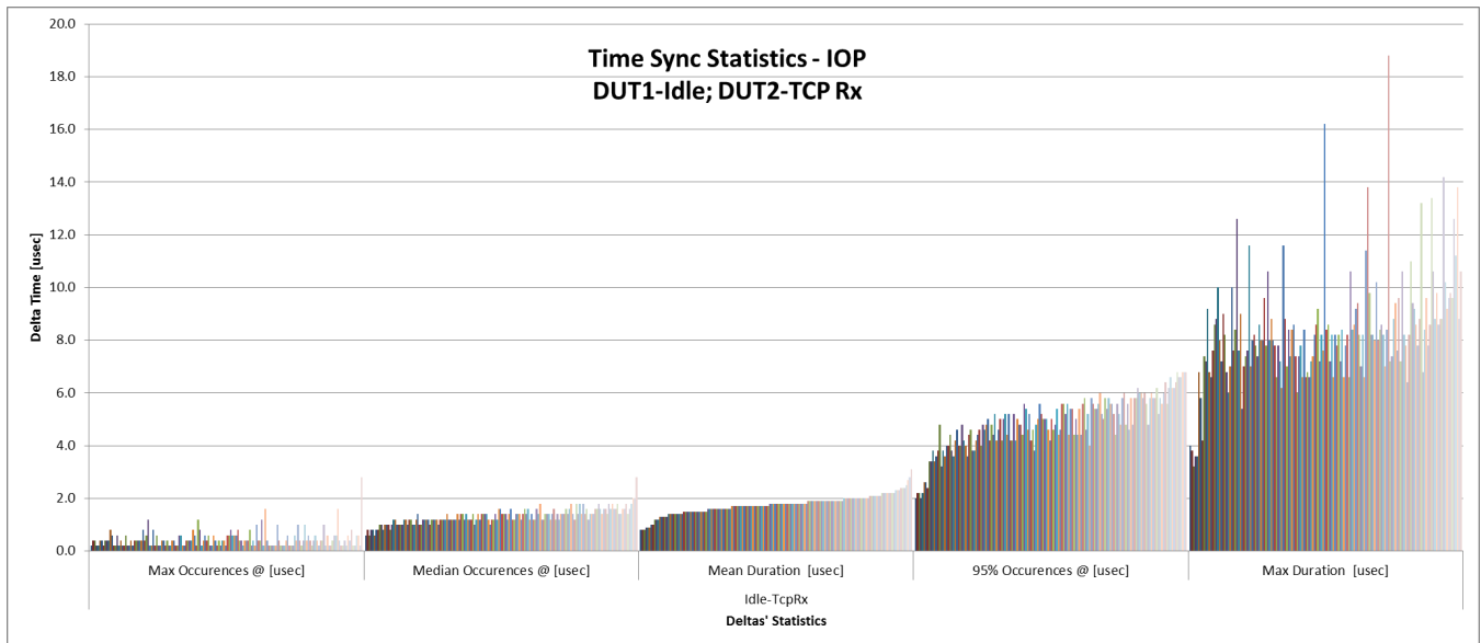
Figure 6. IOP Results –Device 1 Connected Idle, Device 2 is Running TCP Rx
