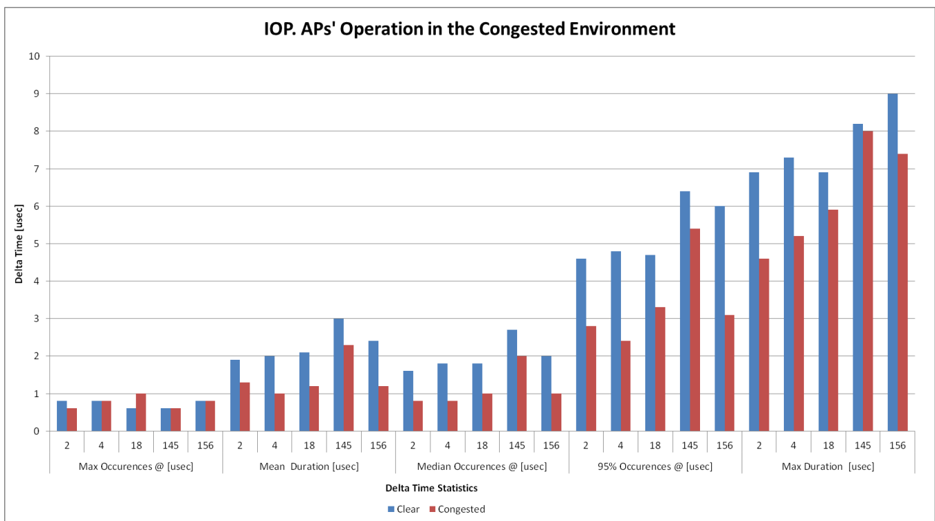
Figure 12. IOP – Clean vs Congested Environment Results
