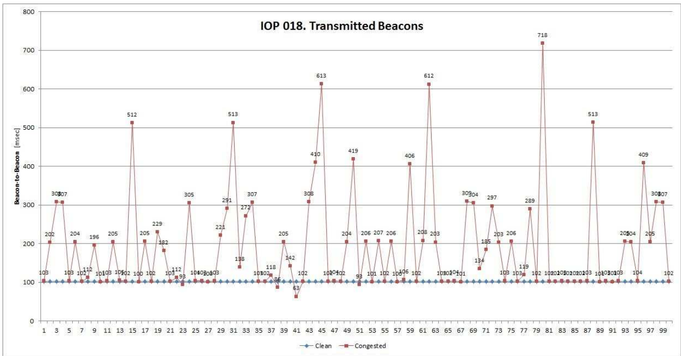
Figure 13. IOP 018 – Beacons Behavior in the Congested Environment
