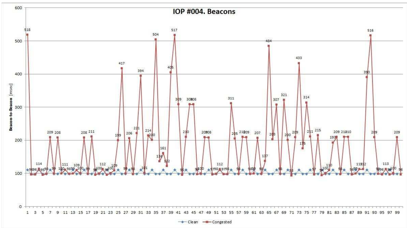
Figure 14. IOP 004 – Beacons Behavior in the Congested Environment
