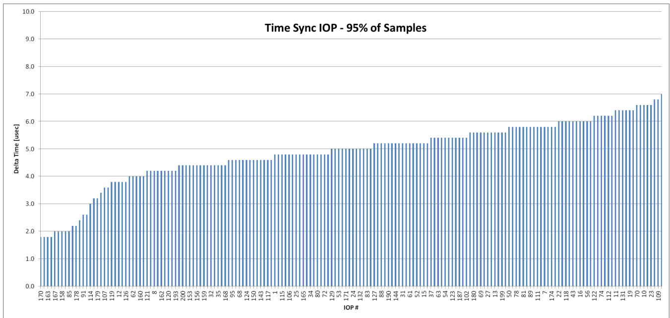
Figure 10. IOP – 95% of all Delta Times Instances Measured Between Two Devices for all APs
